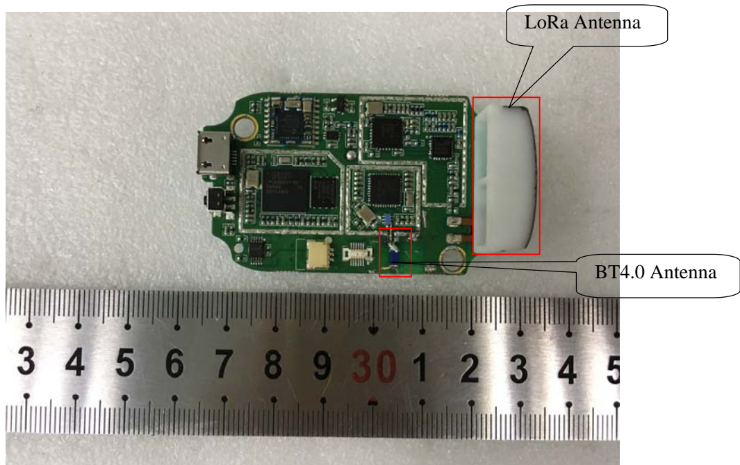
EUT – Main Board Top Shilding off View
