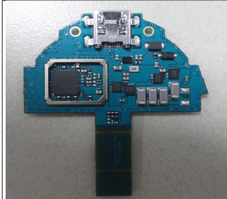
Bottom view of main board
