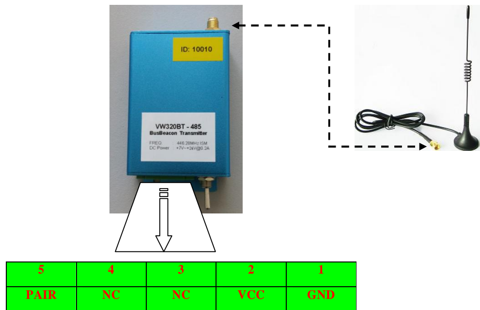
Figure 2: Pin configuration
