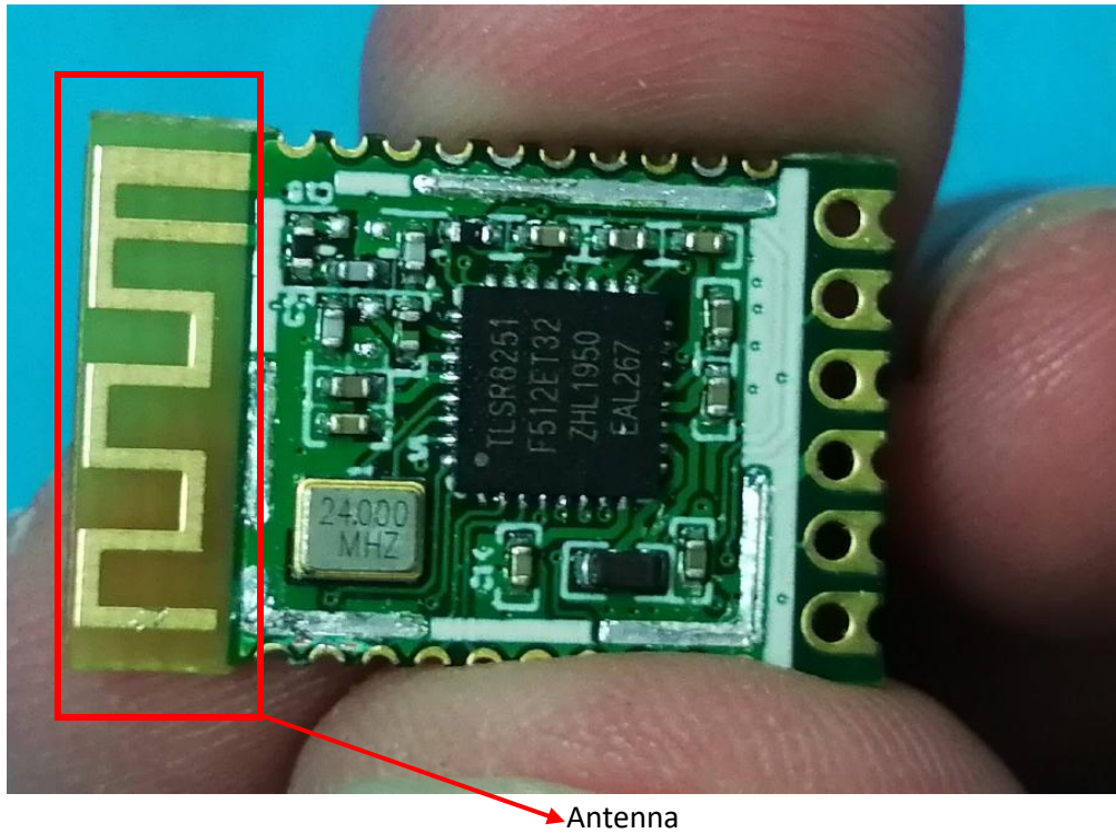
Internal view EUT(HJ8258)
