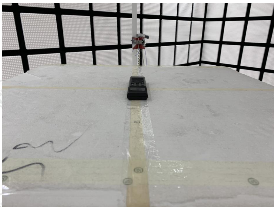
Radiated spurious emission Test Setup-2(Above 1GHz)--HJSR81B Ble
