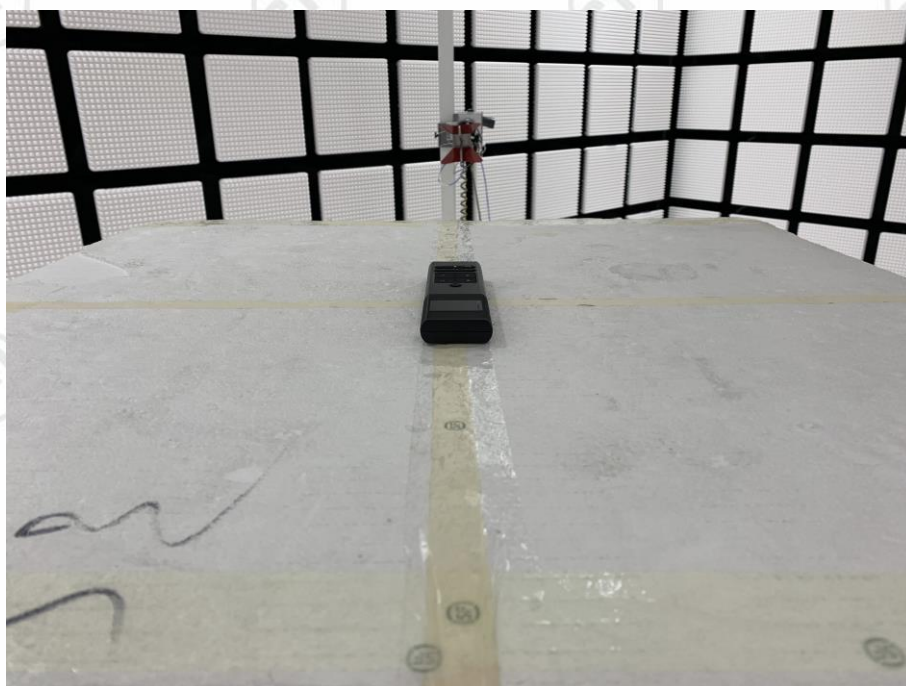
Radiated spurious emission Test Setup-2(Above 1GHz)--HJSR81D Ble
