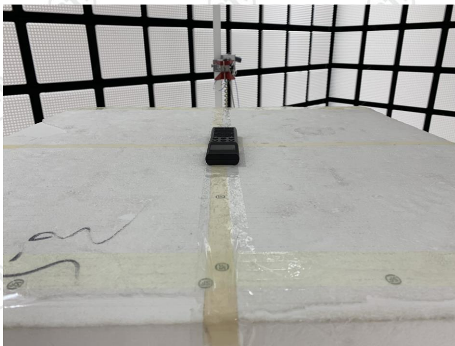
Radiated spurious emission Test Setup-2(Above 1GHz)--HJSR81 Ble
