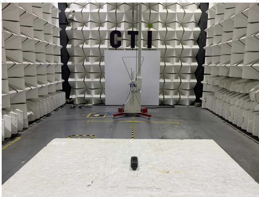
Radiated spurious emission Test Setup-1(Below 1GHz)--HJSR79 Ble
