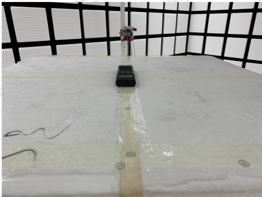
Radiated spurious emission Test Setup-2(Above 1GHz)--HJSR81C Ble
