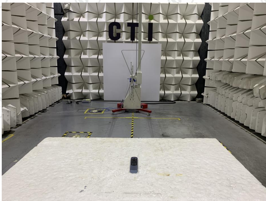
Radiated spurious emission Test Setup-2(Above 1GHz)--HJSR77C Ble
