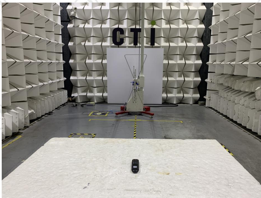
Radiated spurious emission Test Setup-1(Below 1GHz)--HJSR32 Ble
