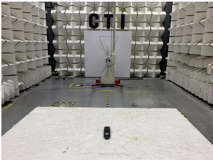
Radiated spurious emission Test Setup-1(Below 1GHz)--HJSR32B Ble
