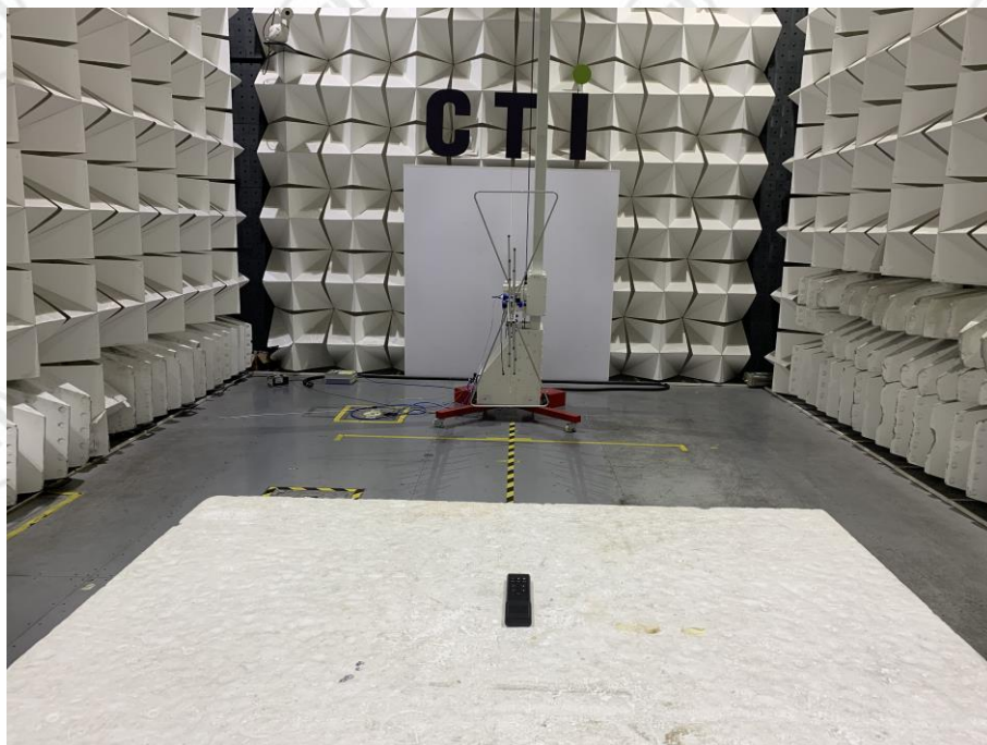
Radiated spurious emission Test Setup-1(Below 1GHz)--HJSR81D Ble
