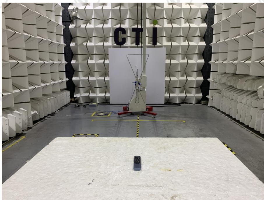
Radiated spurious emission Test Setup-2(Above 1GHz)--HJSR77 Ble
