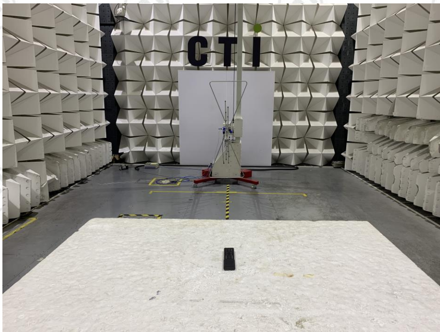
Radiated spurious emission Test Setup-1(Below 1GHz)--HJSR81C Ble
