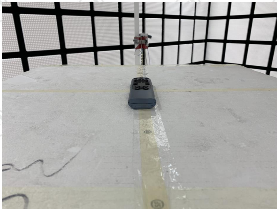
Radiated spurious emission Test Setup-1(Below 1GHz)--HJSR77C Ble
