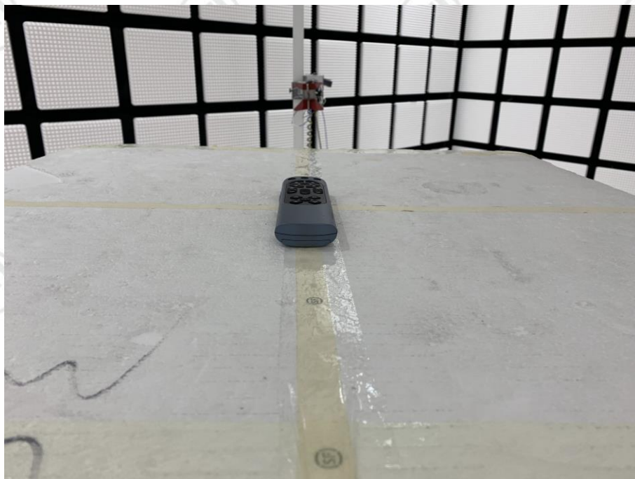
Radiated spurious emission Test Setup-1(Below 1GHz)--HJSR77B Ble
