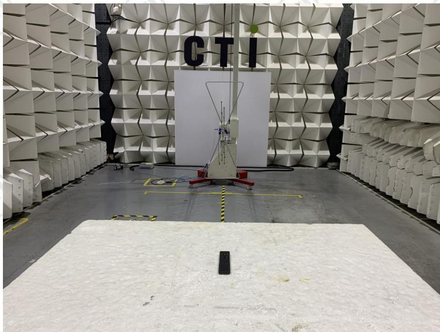
Radiated spurious emission Test Setup-1(Below 1GHz)--HJSR81E Ble
