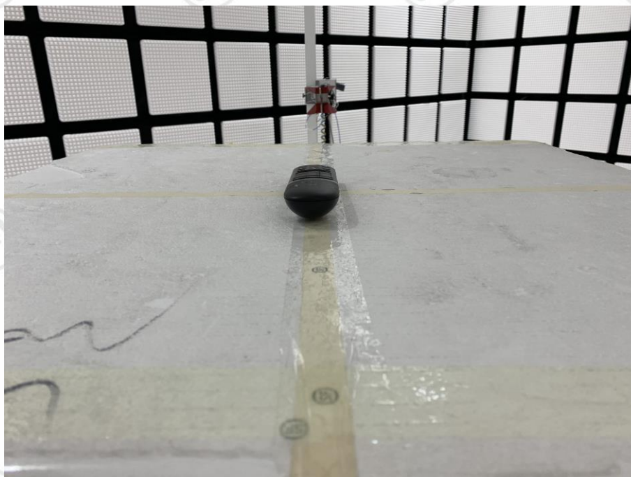
Radiated spurious emission Test Setup-2(Above 1GHz)--HJSR79 Ble
