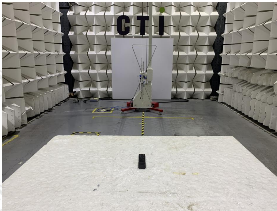
Radiated spurious emission Test Setup-1(Below 1GHz)--HJSR81 Ble
