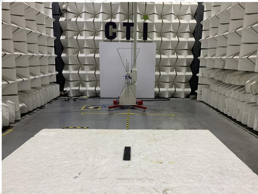
Radiated spurious emission Test Setup-1(Below 1GHz)--HJSR81B Ble
