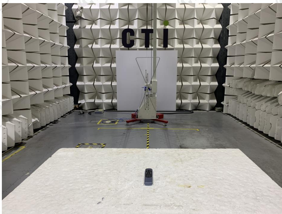
Radiated spurious emission Test Setup-2(Above 1GHz)--HJSR77B Ble
