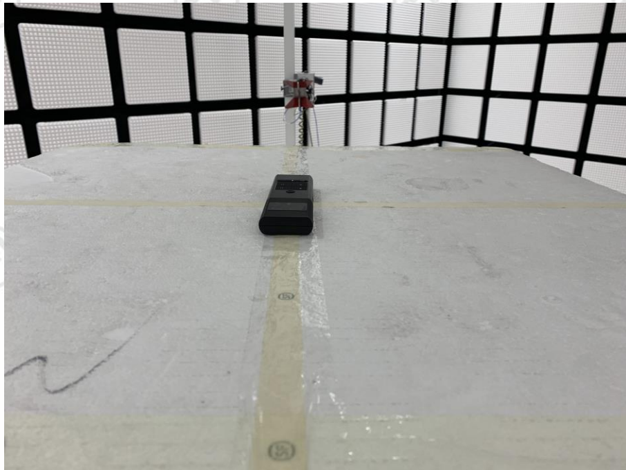
Radiated spurious emission Test Setup-2(Above 1GHz)--HJSR81E Ble
