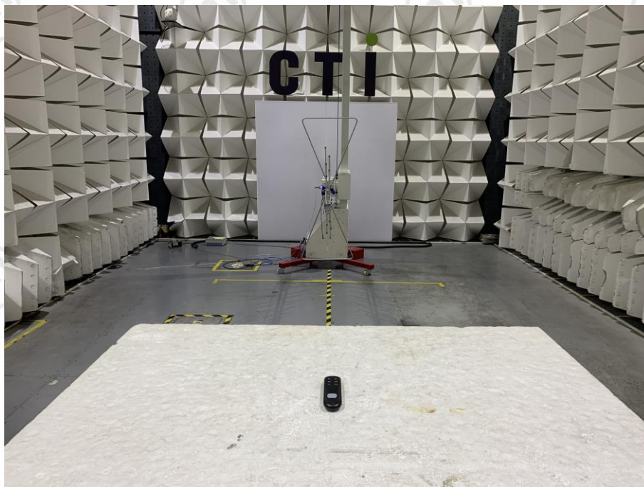
Radiated spurious emission Test Setup-1(Below 1GHz)--HJSR32C Ble
