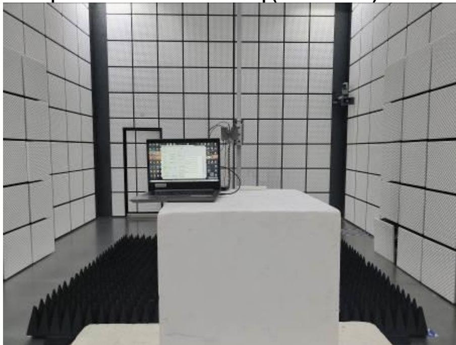
Radiated spurious emission Test Setup(Above 1GHz)-- HJH55BA Ble
