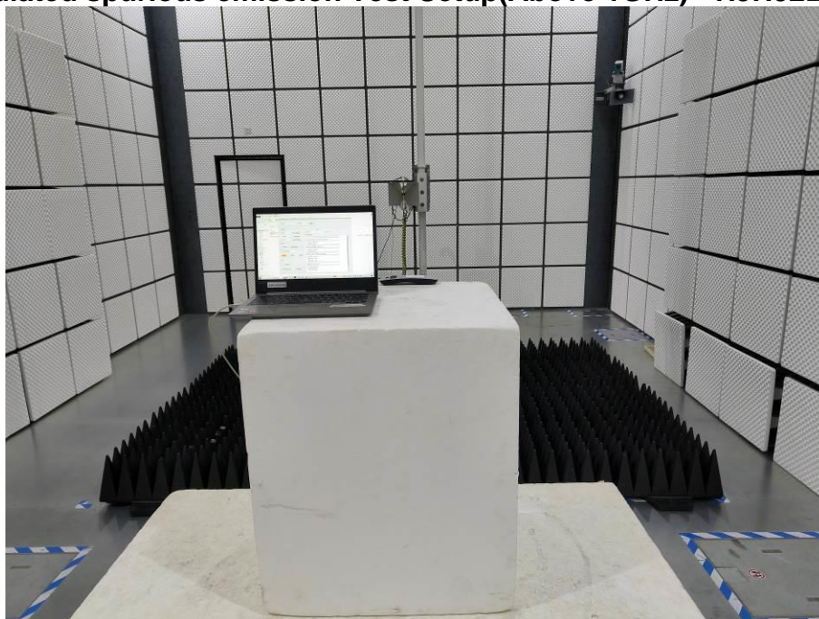
Radiated spurious emission Test Setup(Above 1GHz)-- HJH92B Ble
