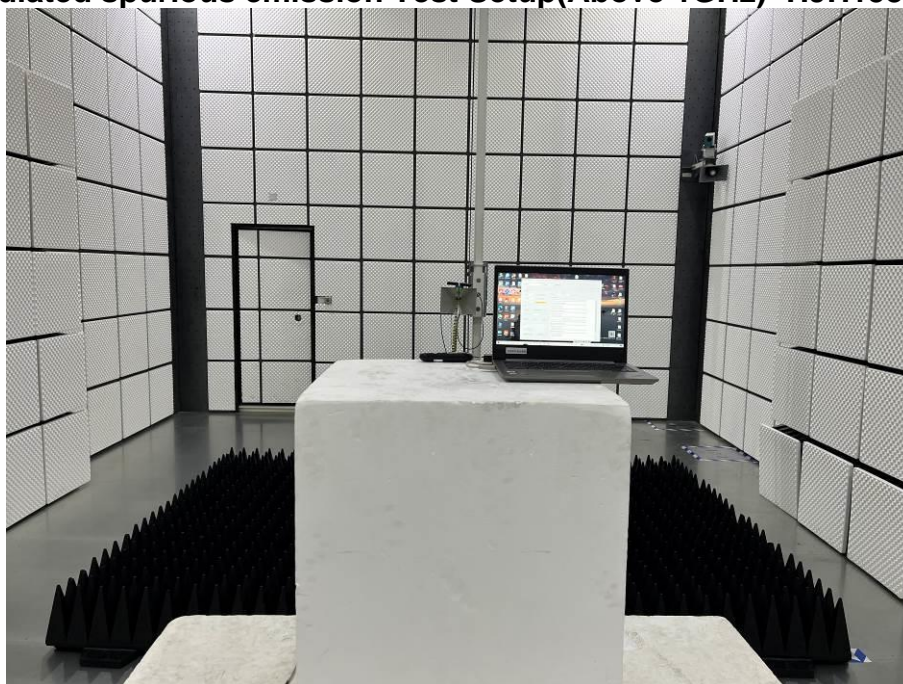
Radiated spurious emission Test Setup(Above 1GHz)- HJH158 Ble
