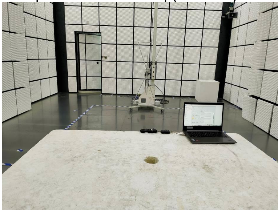
Radiated spurious emission Test Setup (Below 1GHz)- HJH158 Ble
