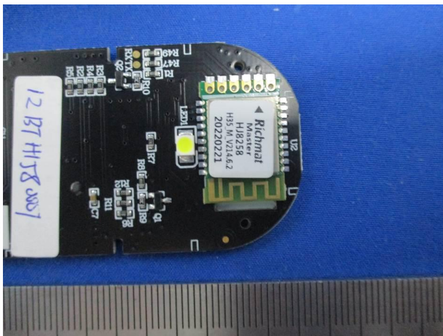
View of Product (HJH158 Ble) -5
