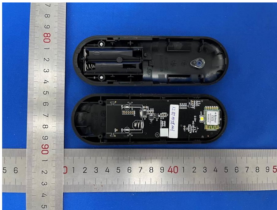
View of Product (HJH158 Ble) -1
