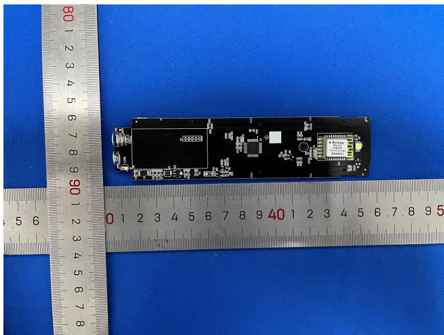
View of Product (HJSR69 Ble) -13
