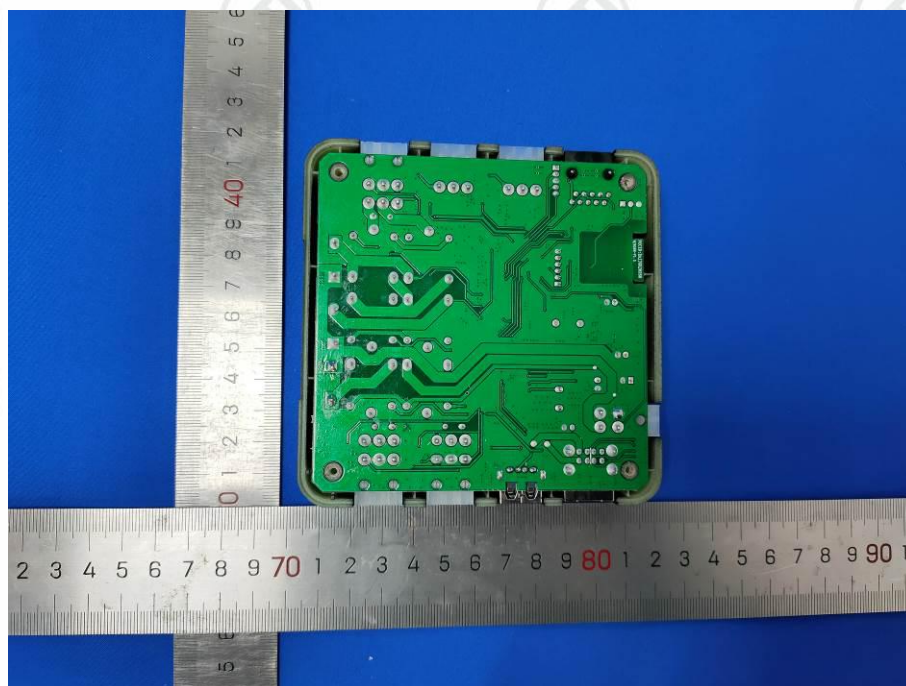
View of Product (HJC26C Ble) -7
