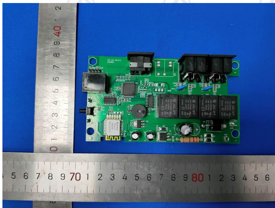
View of Product (HJC18 Ble) -15
