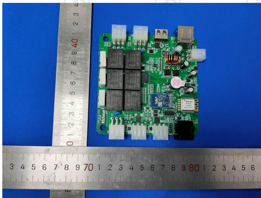
View of Product (HJC26C Ble) -9
