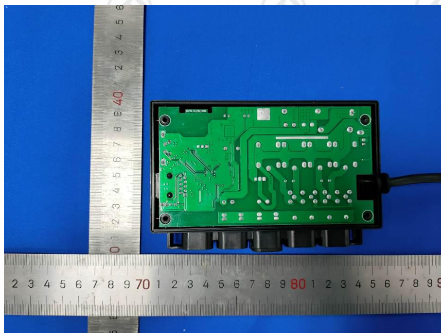
View of Product (HJC18 Ble) -13
