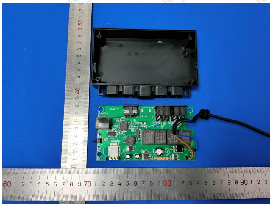
View of Product (HJC18 Ble) -14
