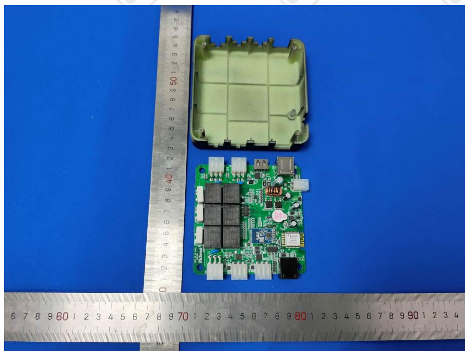
View of Product (HJC26C Ble) -8
