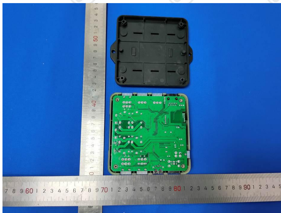
View of Product (HJC26C Ble) -6
