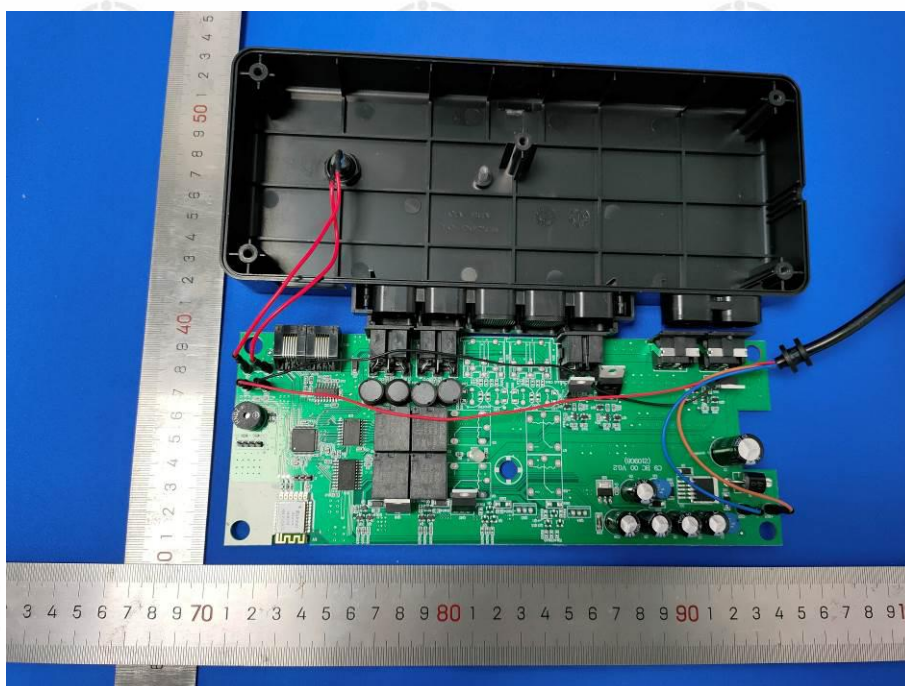
View of Product (HJC9G Ble) -2
