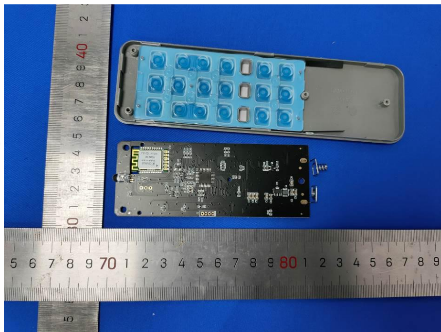
View of Product (HJH55 Ble) -8
