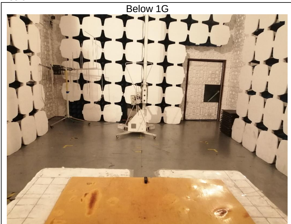
Radiated Emission
