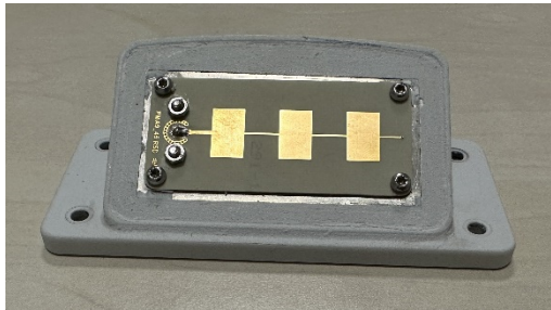
PM Antenna fixed on the support
