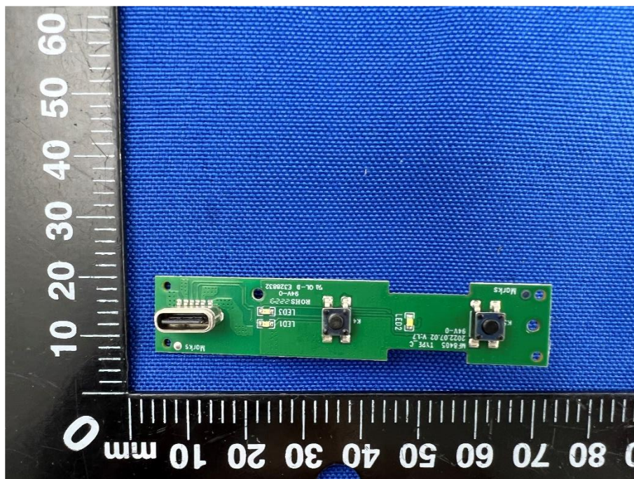
USB BOARD TOP VIEW
