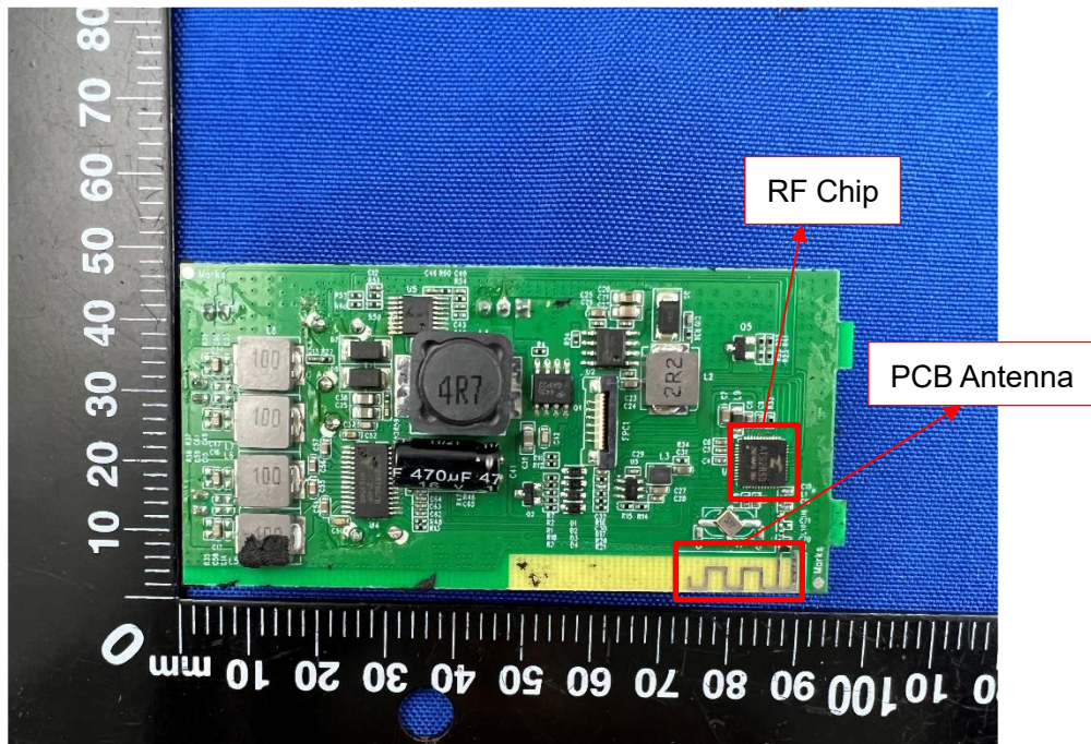
MAIN BOARD TOP VIEW
