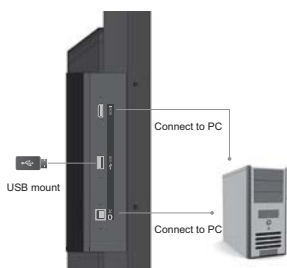
INSTALLATION DIAGRAM OF SIDE PANEL
