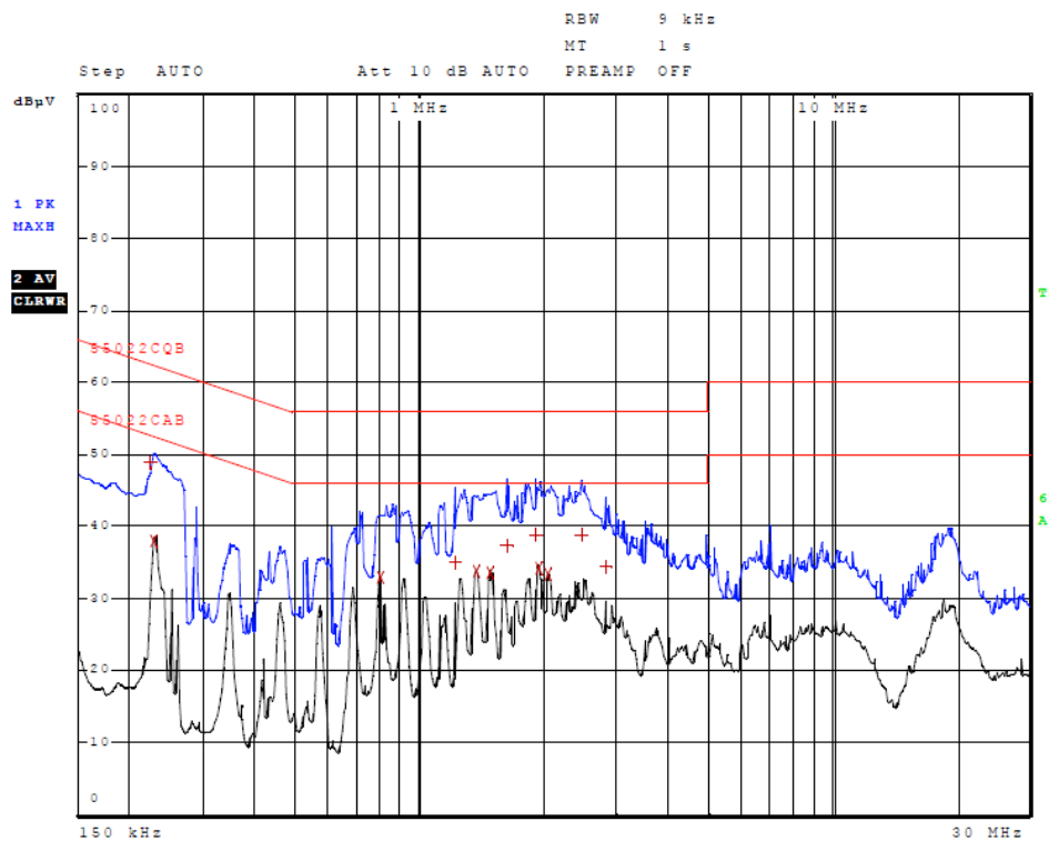
Figure 2 AC Line Conducted emissions of EUT line 2 (EUT USB CPU Adapter)
