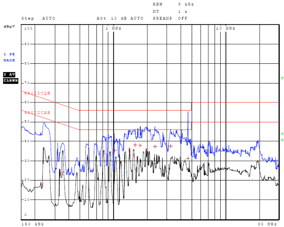
Figure 1 AC Line Conducted emissions of EUT line 1 (EUT USB CPU Adapter)
