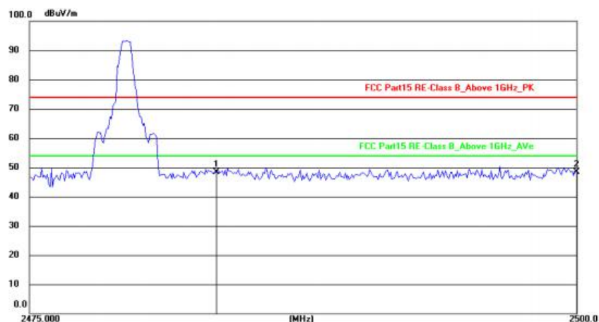
2480MHz Vertical
