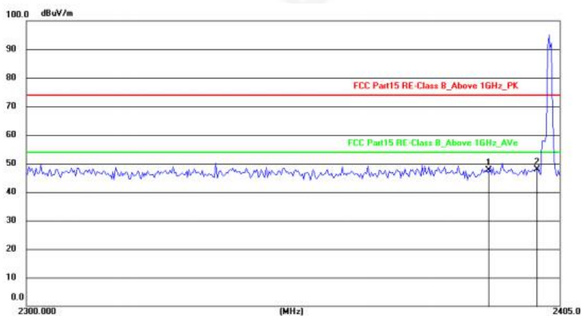
2402MHz Horizontal
