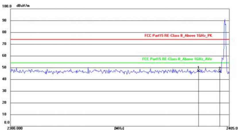
2402MHz Vertical
