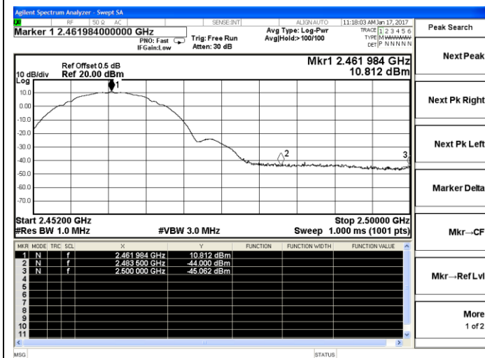
802.11b Chain 0-High channel(Peak)
