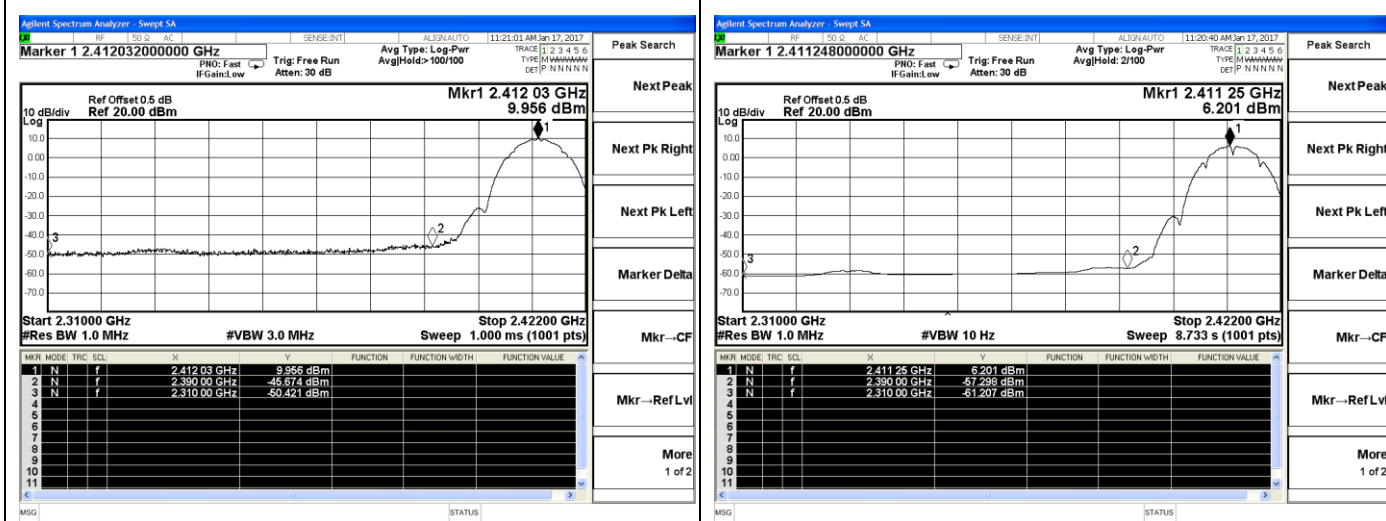
802.11b Chain 0-Low channel(Peak)
