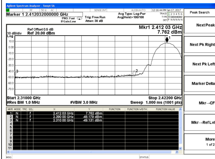
802.11b Chain 1-Low channel(Peak)
