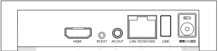
Rear view
