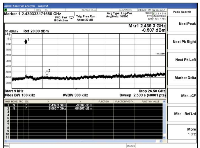
802.11n-HT20-Middle channel
