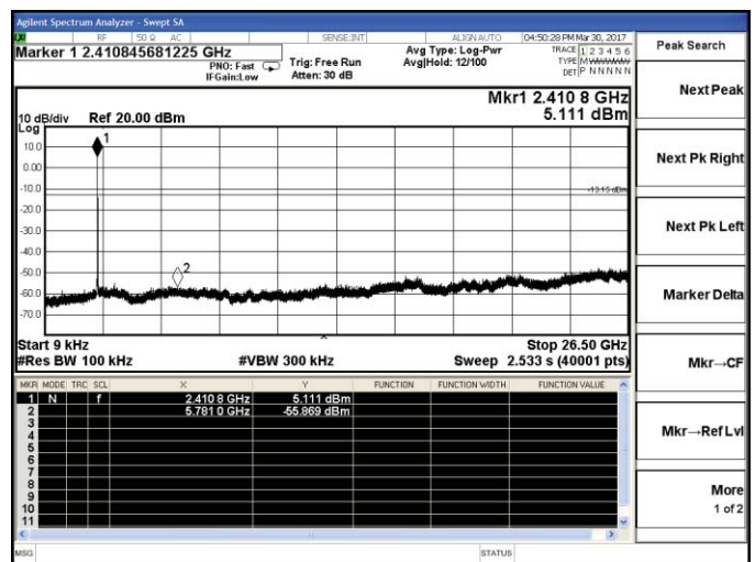
802.11b-Low channel
