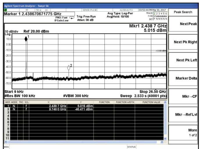
802.11b-Middle channel
