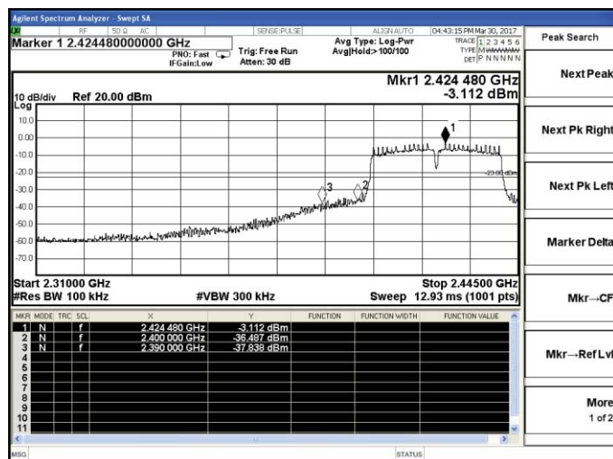
802.11n-HT40-Low channel
