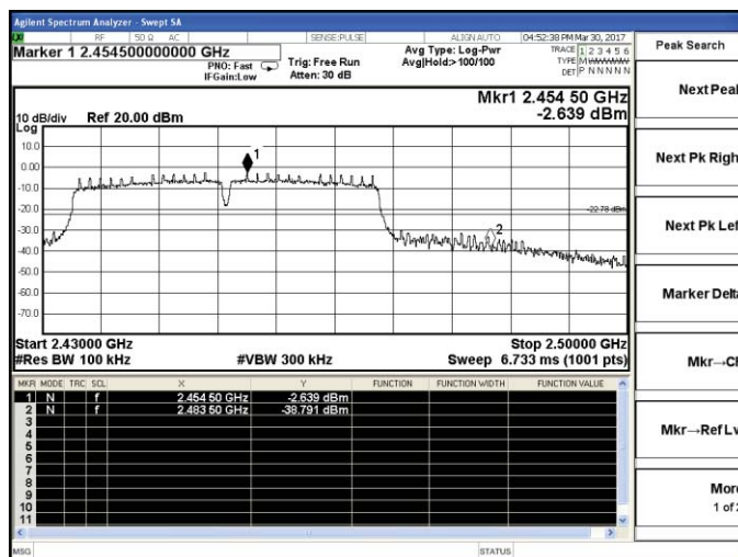
802.11n-HT40-High channel
