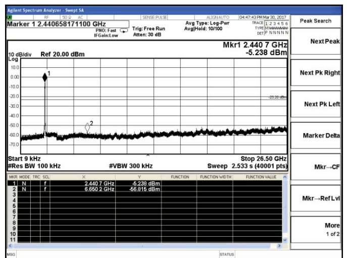
802.11n-HT40-Middle channel
