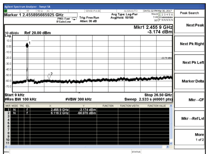
802.11n-HT40-High channel
