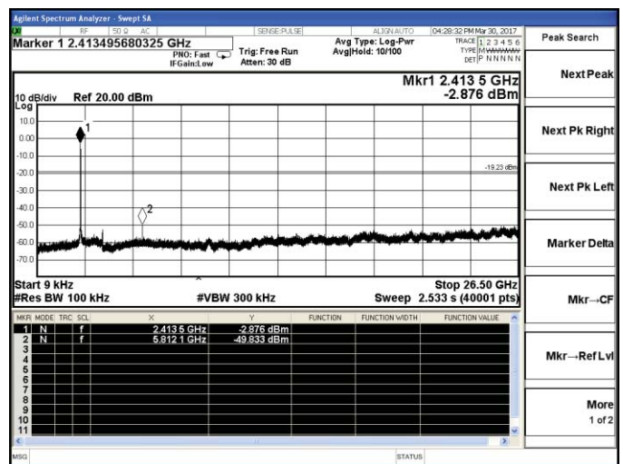
802.11n-HT20-Low channel
