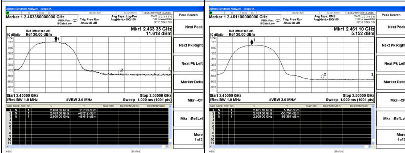
802.11b High channel(Peak)
