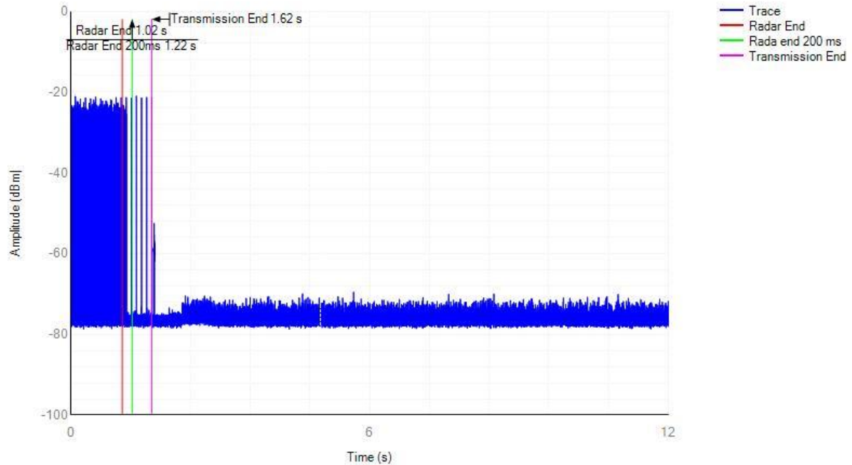
Channel Shutdown
