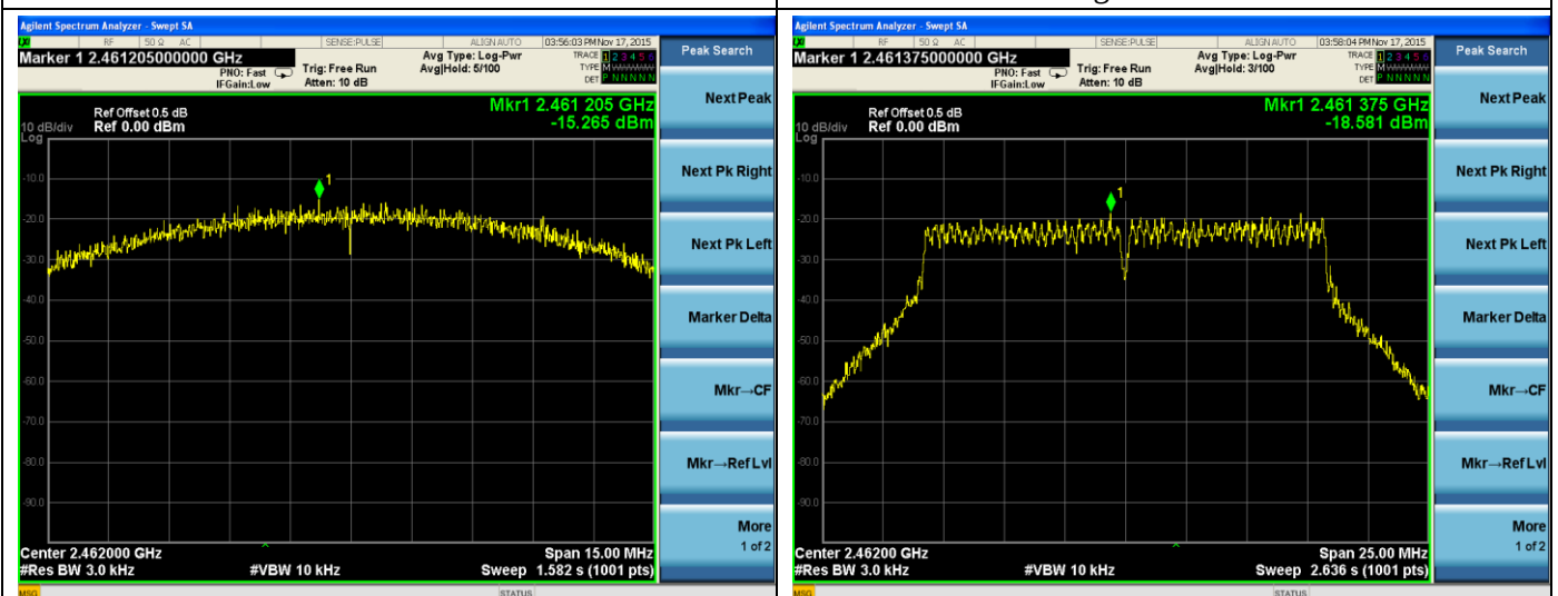
802.11b-High channel
