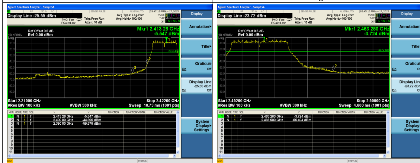
802.11g-Low channel
