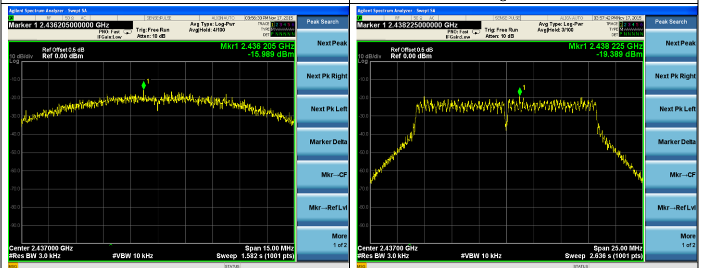
802.11b-Middle channel
