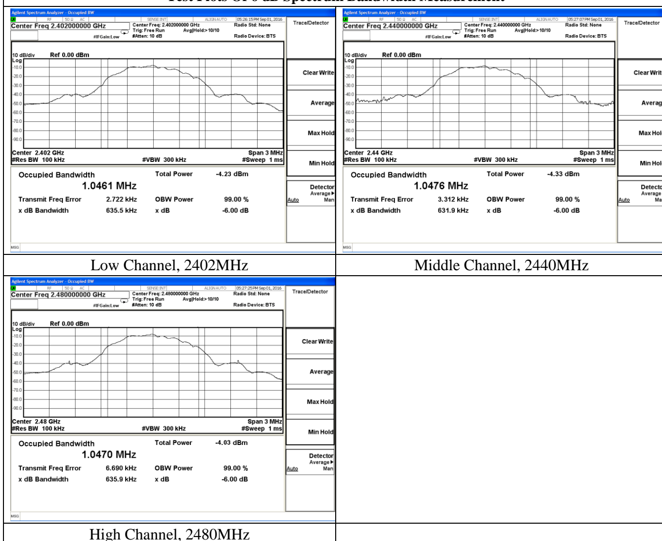
Test Plots Of 6 dB Spectrum Bandwidth Measurement
