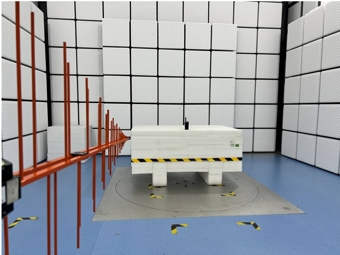
Radiation Emission - Back View (Below 1GHz)
