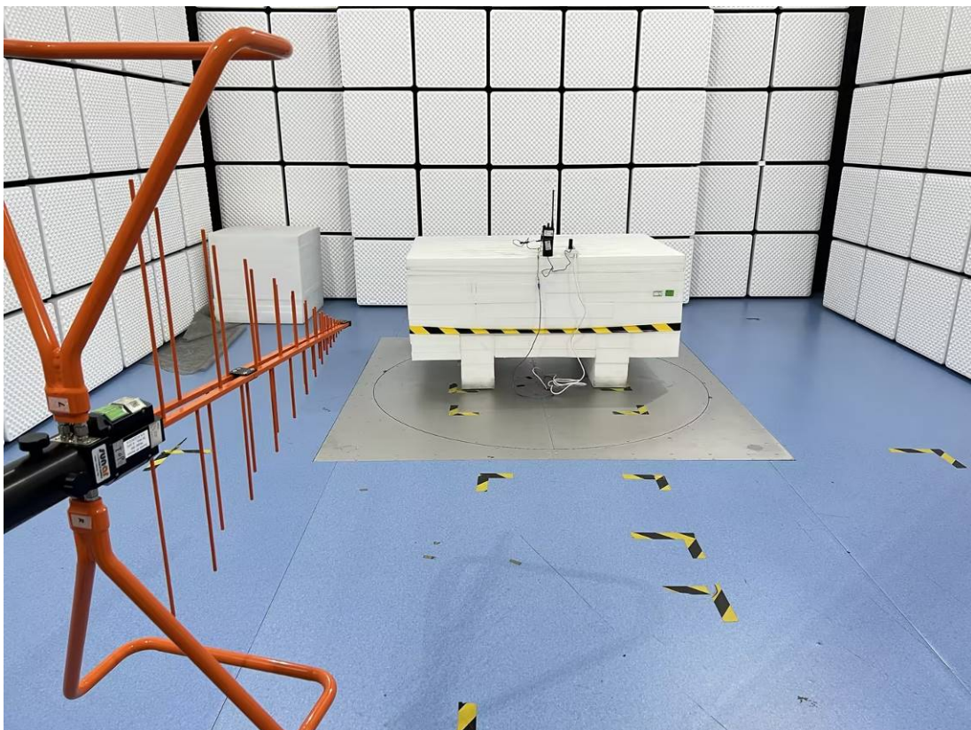
Radiation Emission_30MHz~1GHz - Rear View (Adapter Mode)
