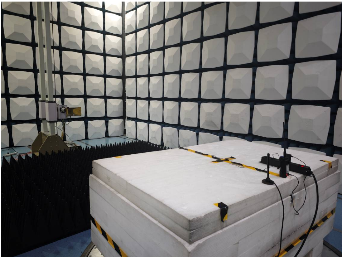
Radiated Emission Above 1GHz Rear View-Antenna 2
