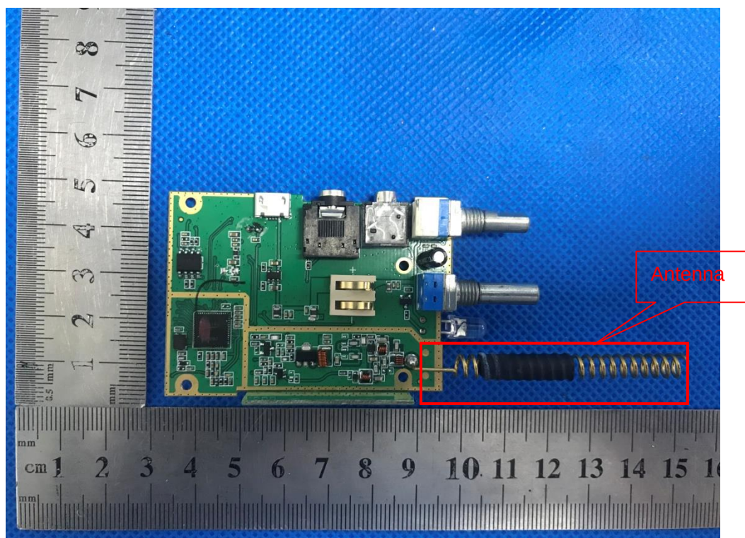
INTERNAL VIEW-1 OF EUT
