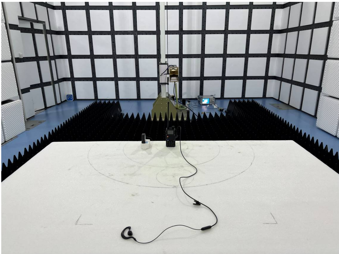
Radiated Emission Above 1 GHz RearView(Test Mode 1)
