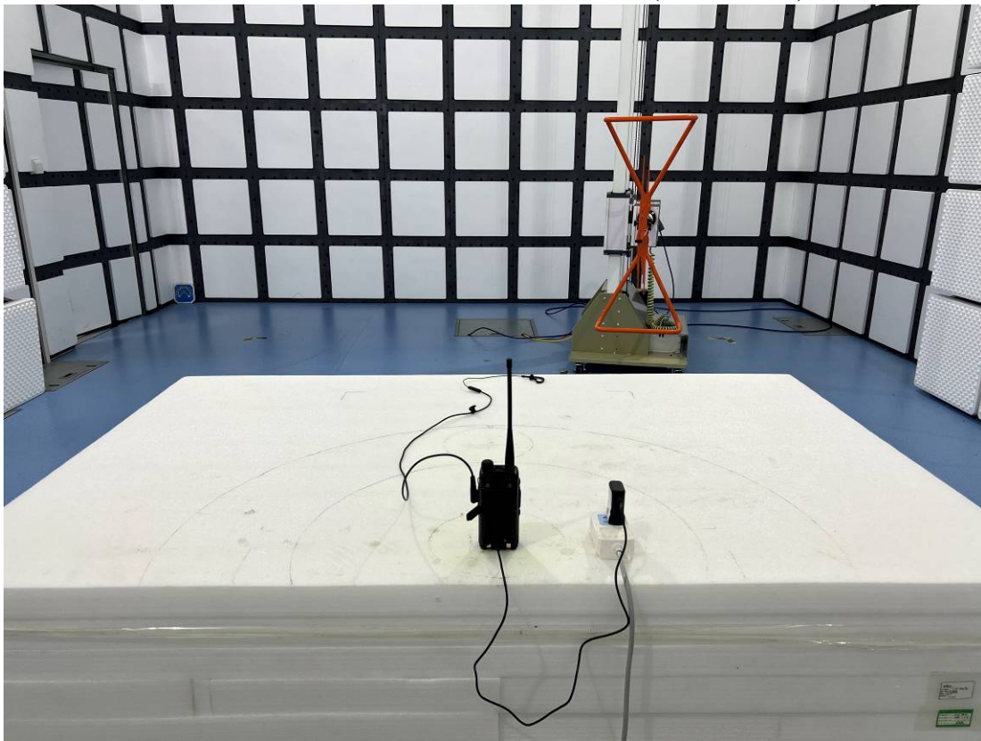
Radiated Emission 30M-1GHz RearView(Test Mode 1)
