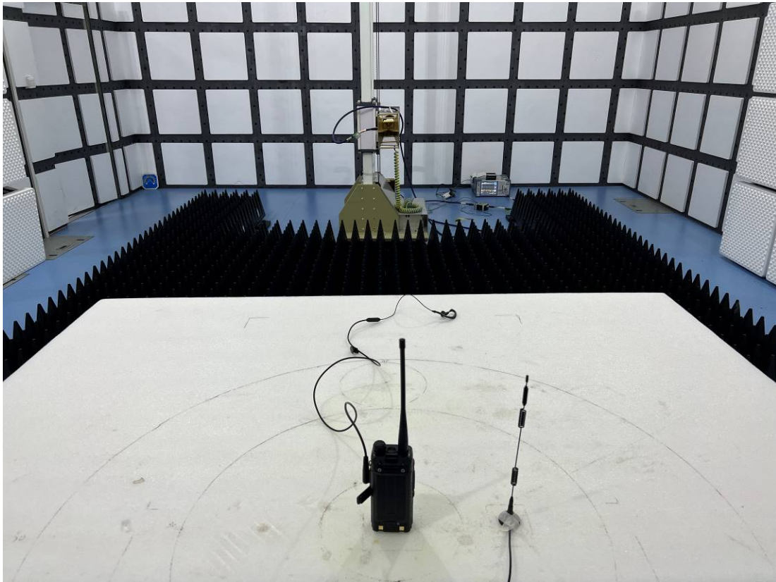
Radiated Emission Above 1 GHz RearView(Test Mode 2)
