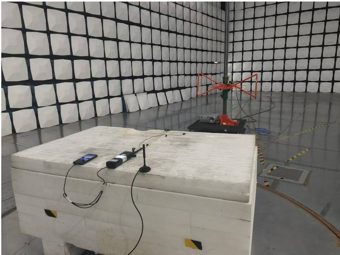
Radiated Emission 30M-1GHz Rear View M3
