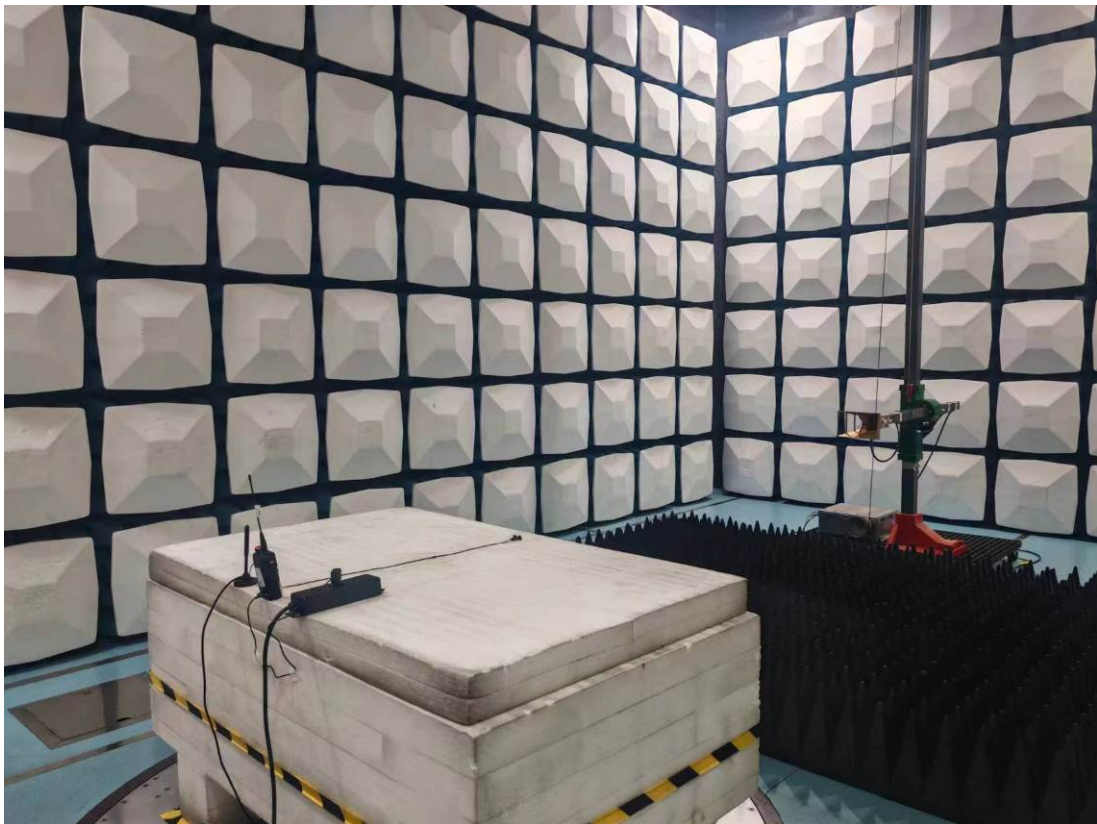
Radiated Emission Above 1GHz Rear View-M1&M2
