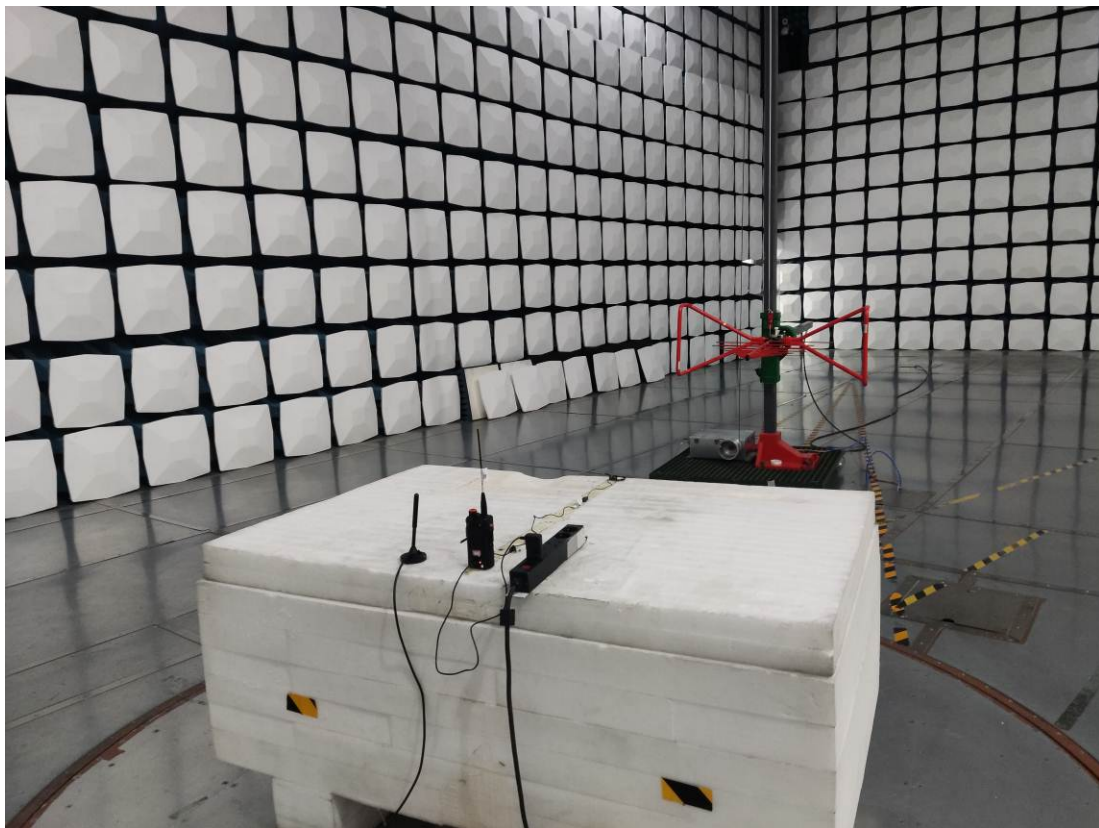
Radiated Emission 30M-1GHz Rear View-M1&M2
