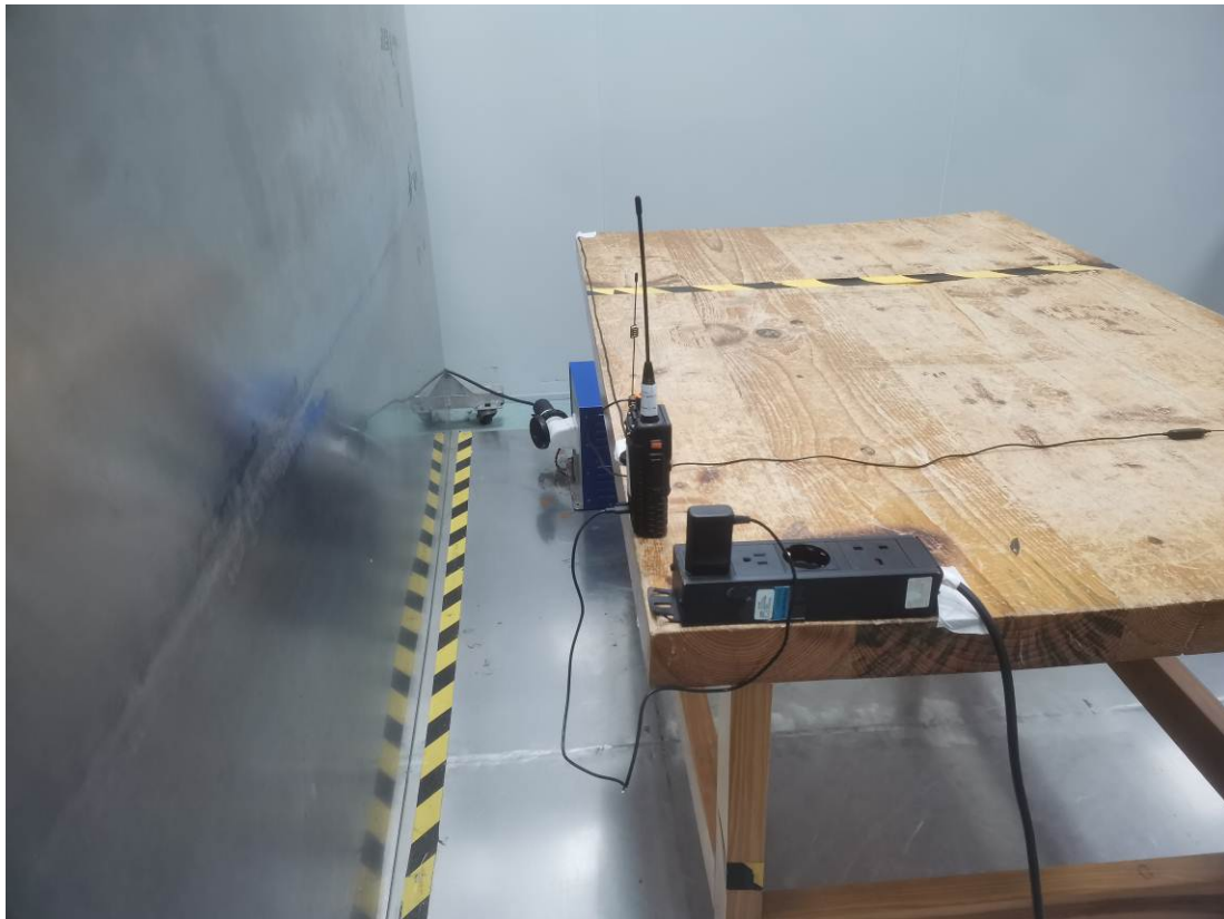
Conducted Emissions Side View-M1&M2
