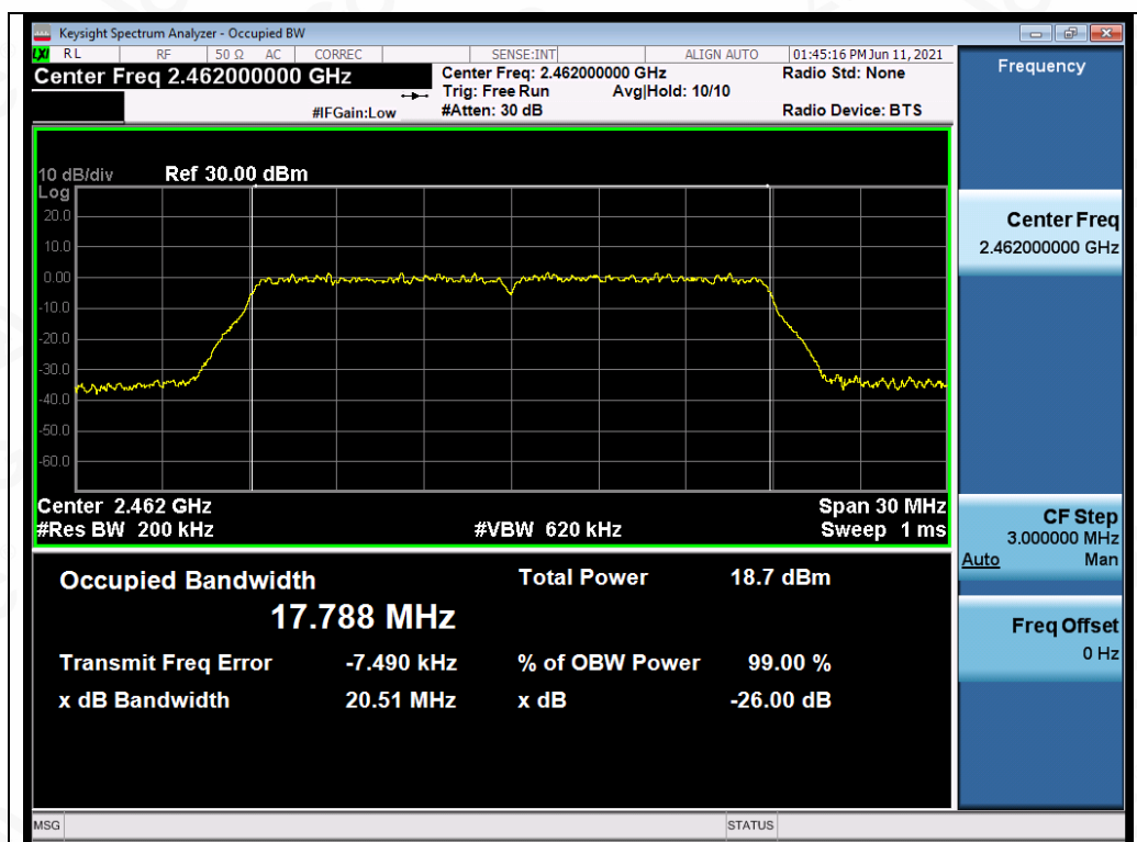
Test_Graph_802.11n20_ANT1_2462_MCS0_OBW
