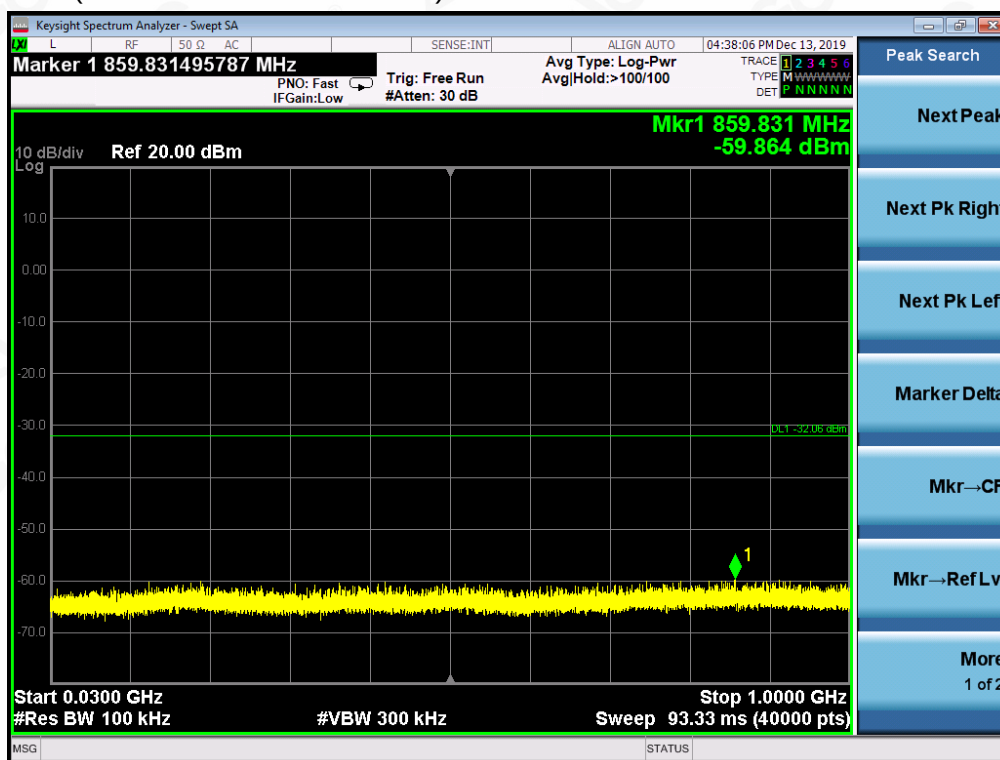
TEST PLOT OF OUT OF BAND EMISSIONS THE WORST CASE OF (802.11n20 with data rate 6.5) FOR MODULATION IN MIDDLE CHANNEL
