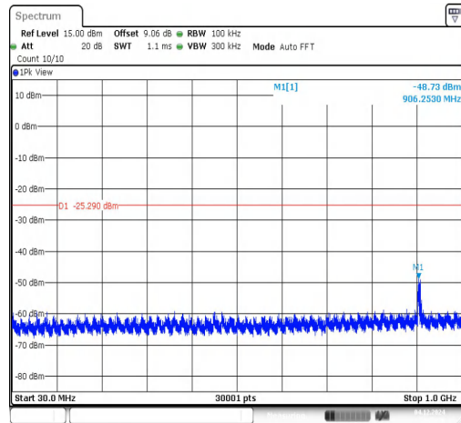
BLE_1M-Ant1-2480-30~1000-PASS
