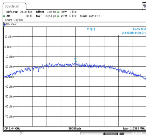
BLE_1M-Ant1-2440-PASS
