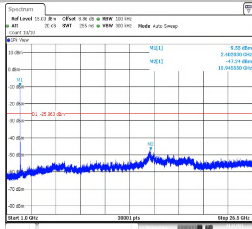
BLE_2M-Ant1-2402-0~Reference-PASS
