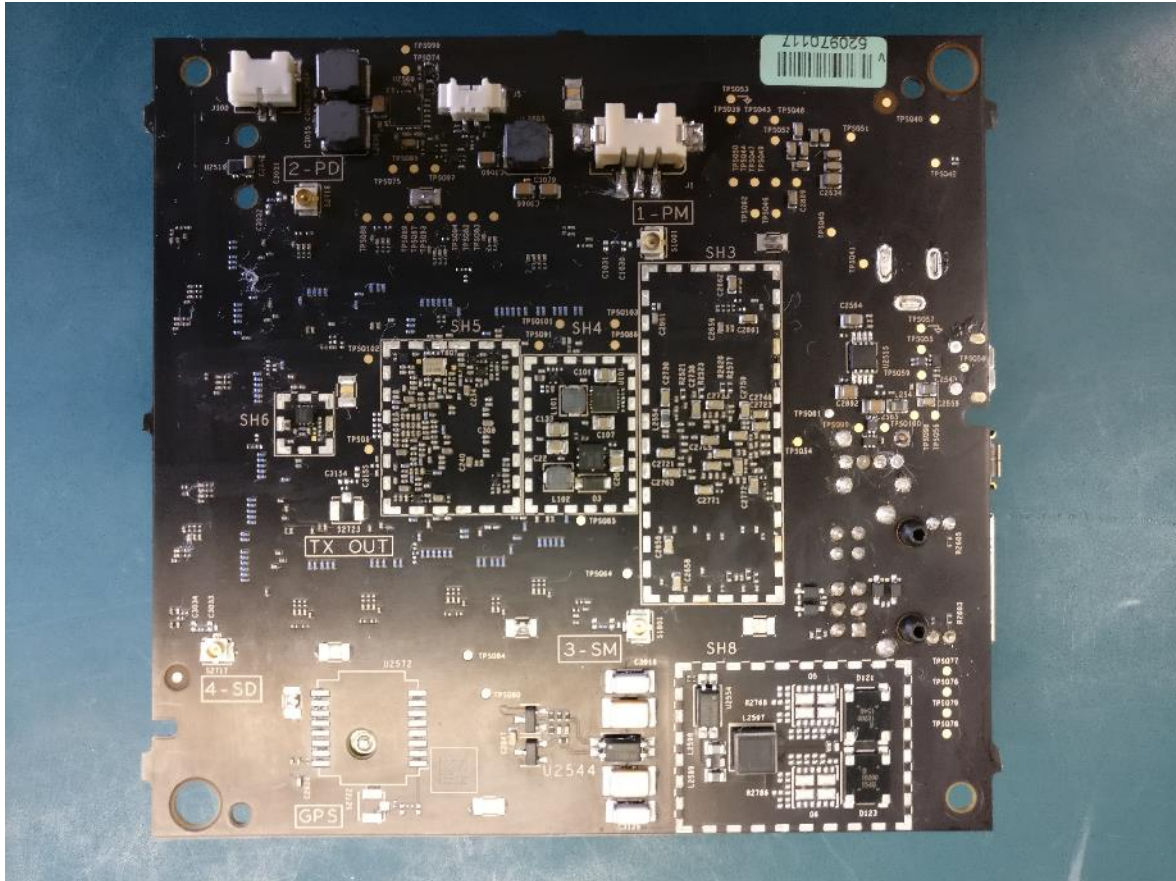
Figure 4 – EUT Internal Photo Bottom (Without the Shields)
