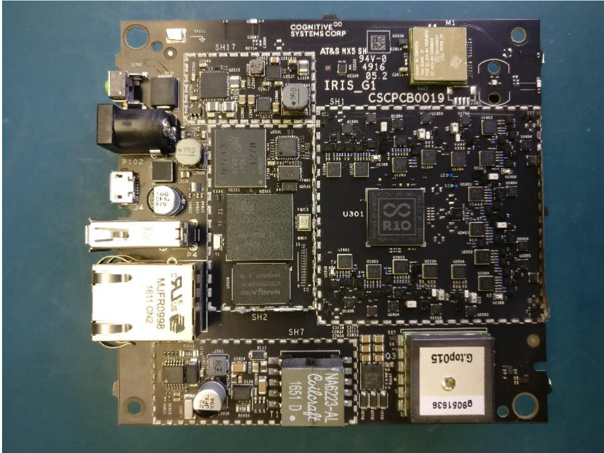
Figure 2 – EUT Internal Photo Top (Without the Shields)
