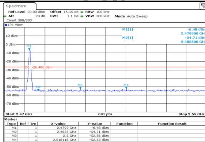
DH1_Ant1_High_2480
