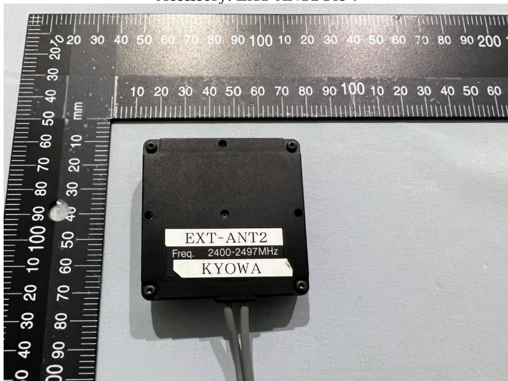
Accessory: EXT-ANT2 Pic 4
