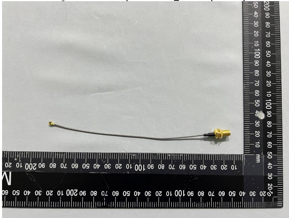
Accessory: AA-562-2020(SMA-MHF_harness(150mm) Pic 1
