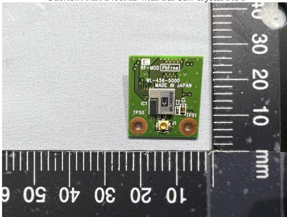
Outview: MR-2400MB with Tai-Saw crystal Pic 1
