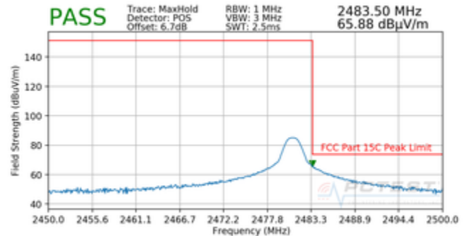
Plot 7-12. Radiated Restricted Upper Band Edge Measurement (Peak) – EX600-WPN1
