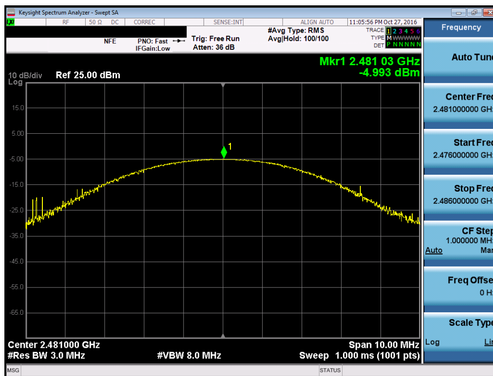
Plot 7-15. Peak Conducted Power (EX600-WEN3-X40, Ch. 78)
