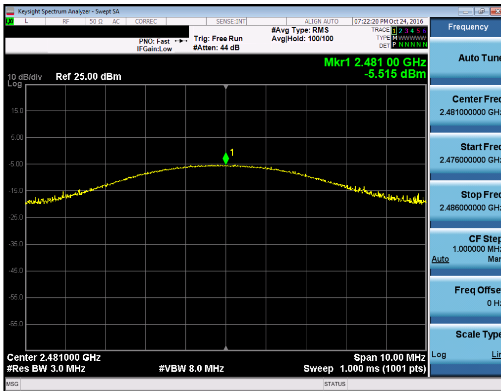
Plot 7-18. Peak Conducted Power (EX600-WEN4-X40, Ch. 78)
