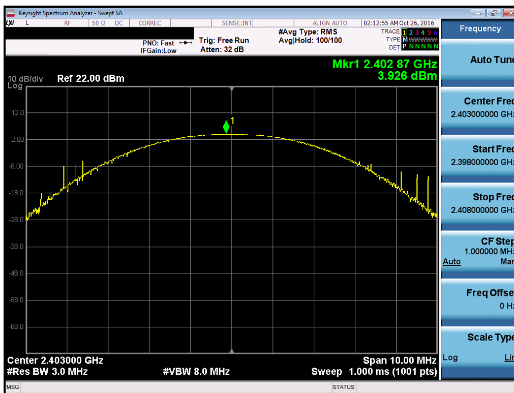
Plot 7-19. Peak Conducted Power (EX600-WSV3-X41, Ch. 0)
