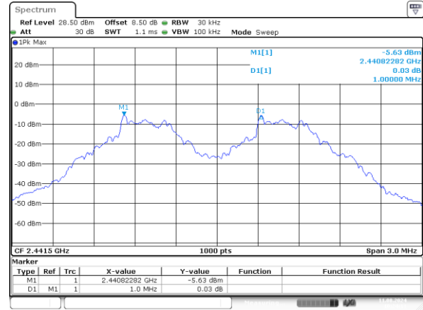
GFSK_Middle 1MHz
