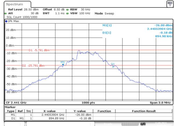
GFSK_Middle 0.895MHz
