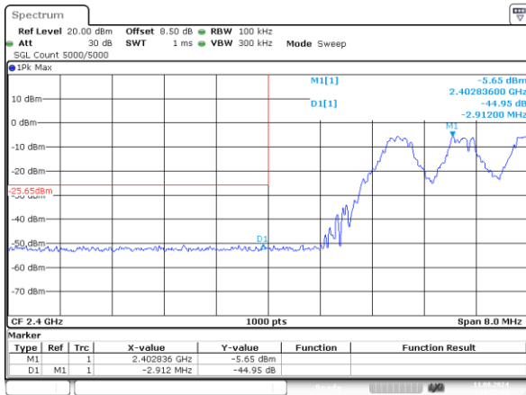
GFSK_Hopping_Lower 44.95dB
