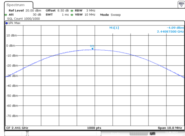
GFSK_Middle -4.09dBm
