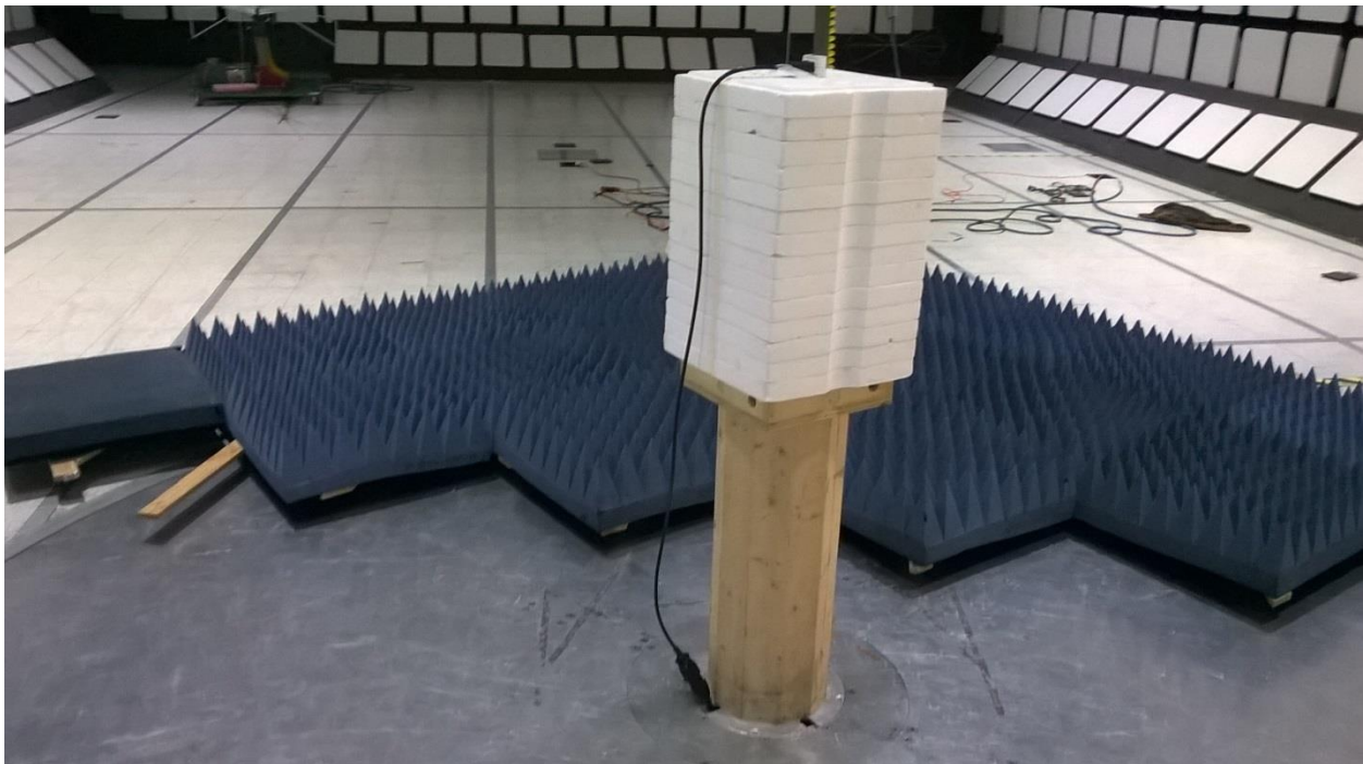
Figure 4 - Test Setup for 1 - 25 GHz, Horizontal Orientation
