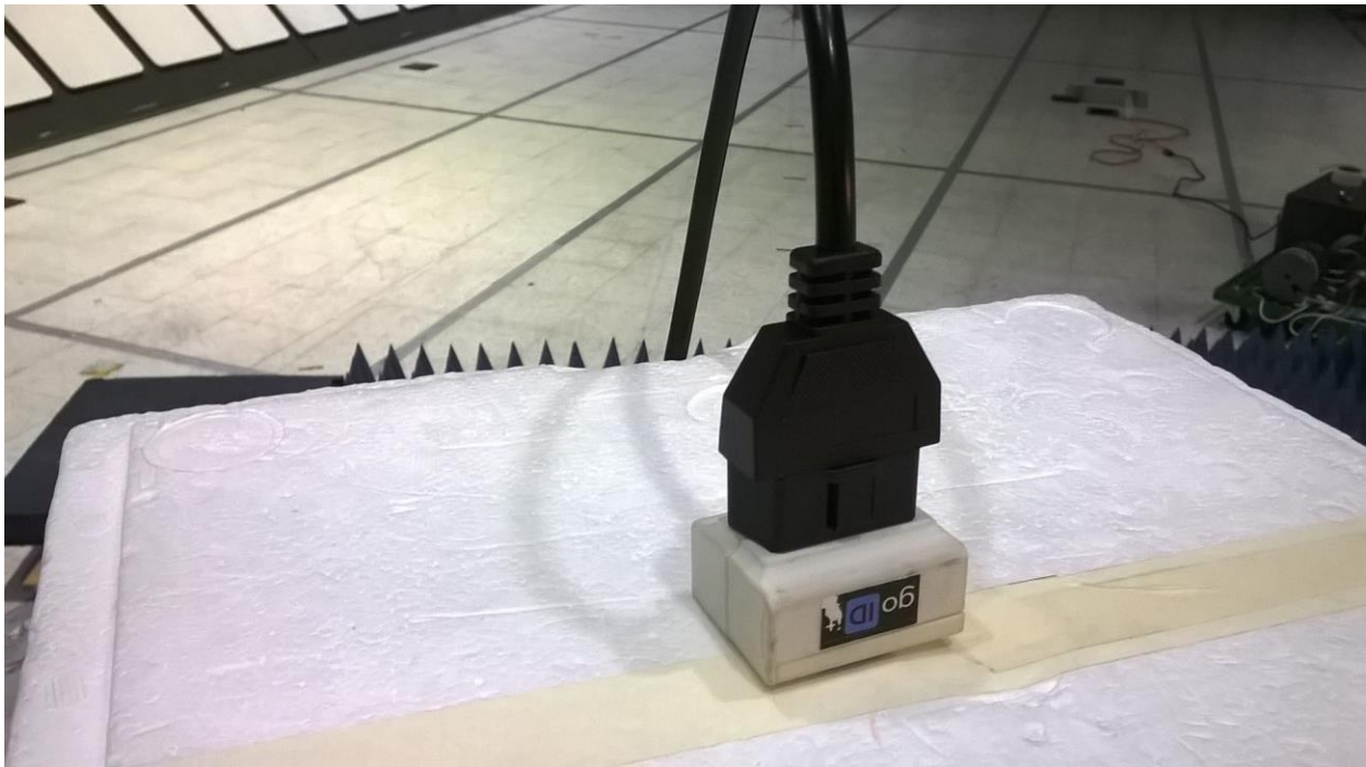
Figure 2 - Radiated Emissions Test Setup, Y-axis
