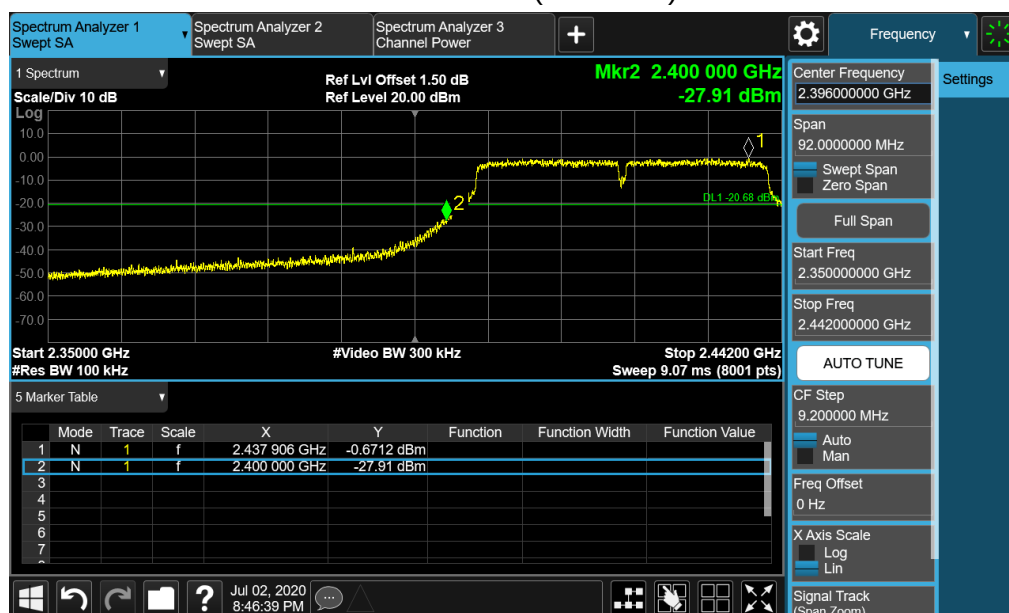
Mode 4 CH03(2422MHz)
