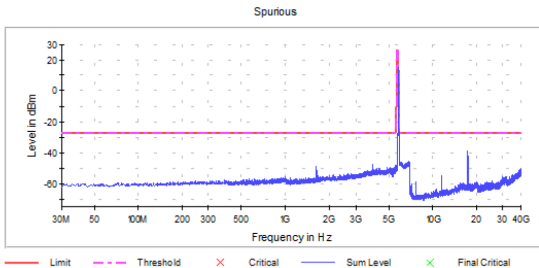
Graph 31: Antenna 1 – Spurious Emissions Channel 165 Transmitting (5825 MHz) - Setting 20
