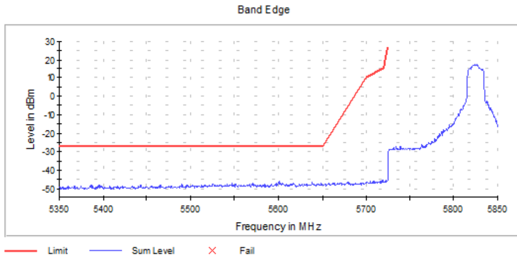
Graph 24: Antenna 1 – Lower Band Edge Channel 165 Transmitting (5825 MHz) - Setting 20
