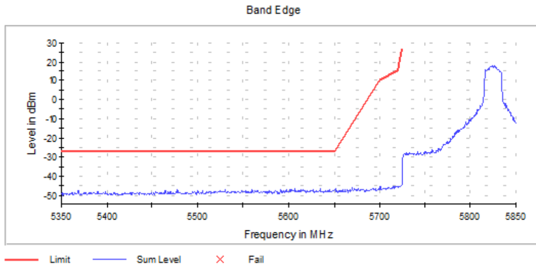
Graph 18: Antenna 0 – Lower Band Edge Channel 165 Transmitting (5825 MHz) - Setting 20
