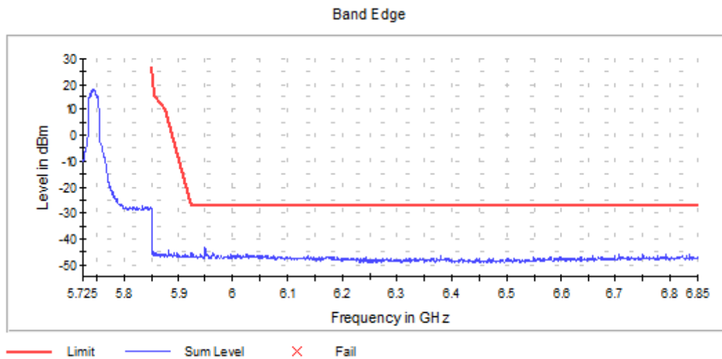
Graph 15: Antenna 0 – Upper Band Edge Channel 149 Transmitting (5745 MHz) - Setting 20
