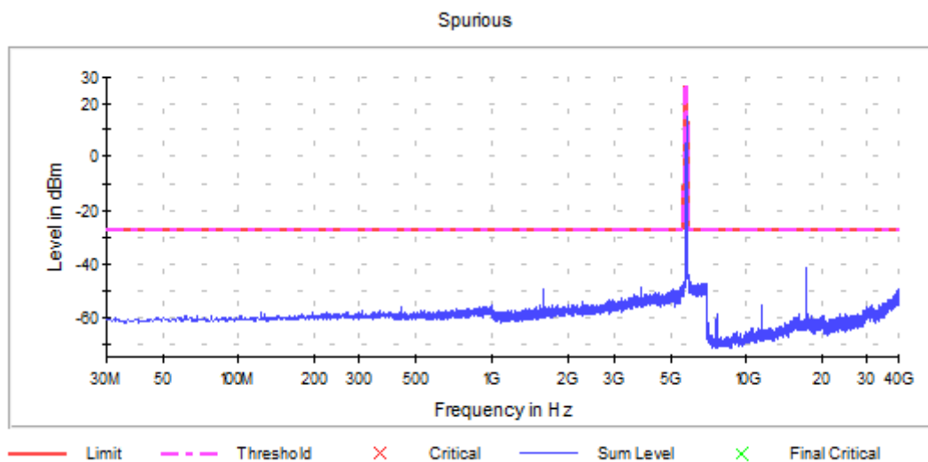
Graph 27: Antenna 0 – Spurious Emissions Channel 157 Transmitting (5785 MHz) - Setting 20
