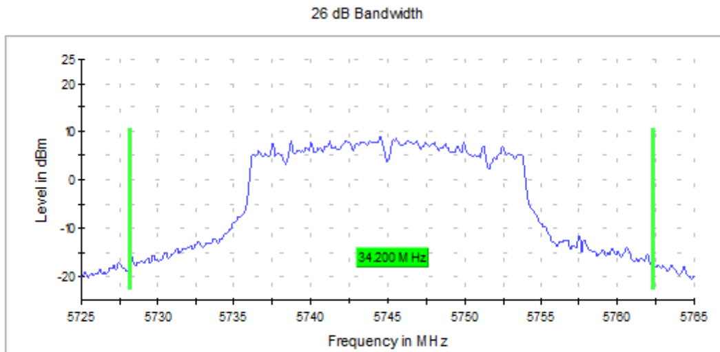
Graph 2: Antenna 0 – 26 dB Emissions Bandwidth Transmitting at 5745 MHz – Setting 20
