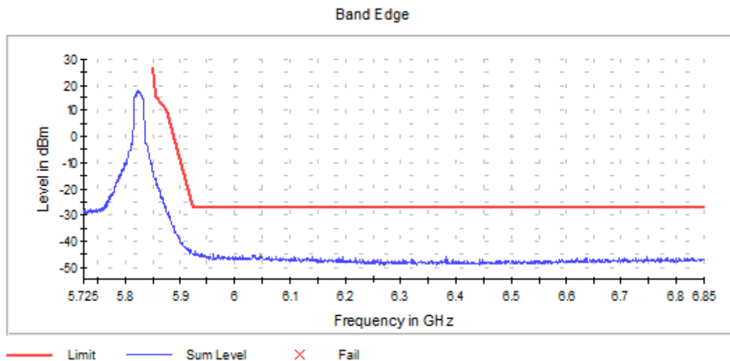
Graph 19: Antenna 0 – Upper Band Edge Channel 165 Transmitting (5825 MHz) - Setting 20
