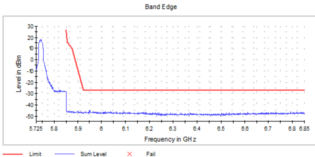
Graph 21: Antenna 1 – Upper Band Edge Channel 149 Transmitting (5745 MHz) - Setting 20
