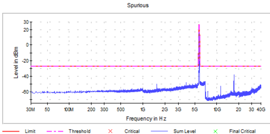
Graph 29: Antenna 1 – Spurious Emissions Channel 149 Transmitting (5745 MHz) - Setting 20
