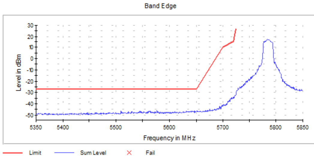
Graph 22: Antenna 1 – Lower Band Edge Channel 157 Transmitting (5785 MHz) - Setting 20
