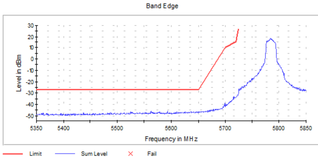
Graph 16: Antenna 0 – Lower Band Edge Channel 157 Transmitting (5785 MHz) - Setting 20
