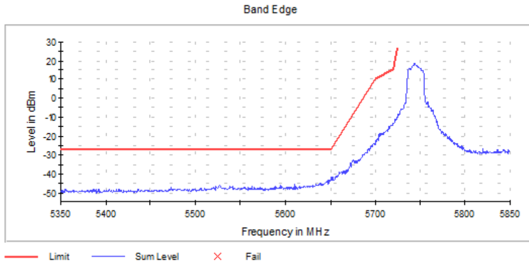
Graph 20: Antenna 1 – Lower Band Edge Channel 149 Transmitting (5745 MHz) - Setting 20
