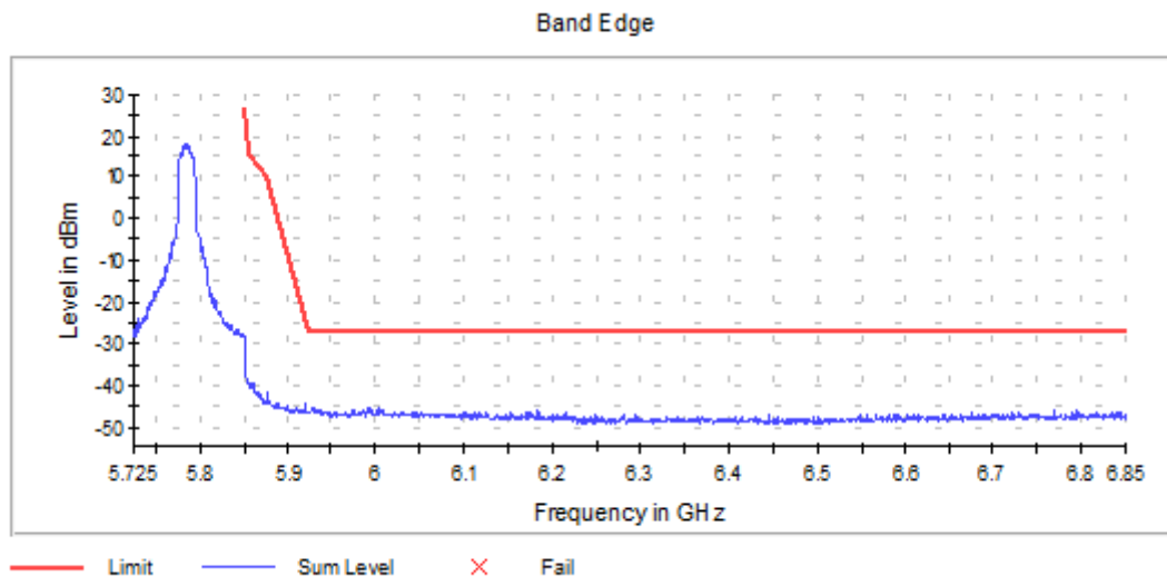
Graph 17: Antenna 0 – Upper Band Edge Channel 157 Transmitting (5785 MHz) - Setting 20
