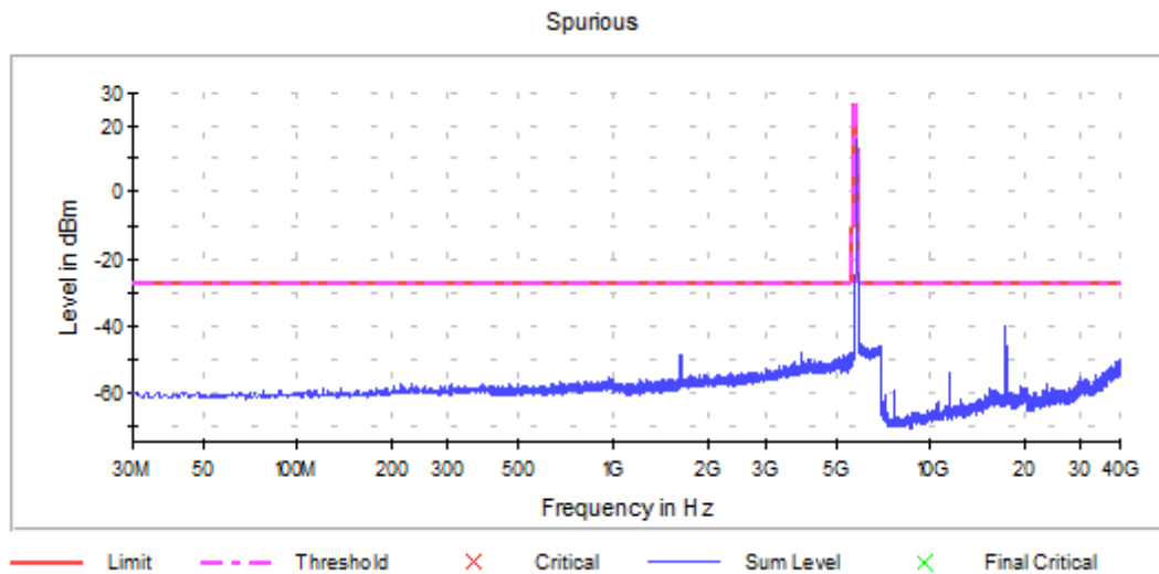
Graph 28: Antenna 0 – Spurious Emissions Channel 165 Transmitting (5825 MHz) - Setting 20
