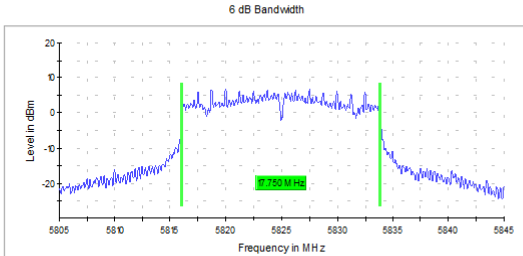
Graph 10: Antenna 0 – 6 dB Emissions Bandwidth Transmitting at 5825 MHz - Setting 20
