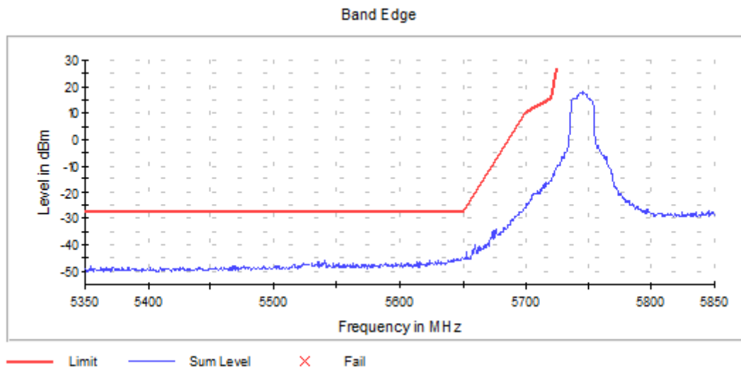
Graph 14: Antenna 0 – Lower Band Edge Channel 149 Transmitting (5745 MHz) - Setting 20
