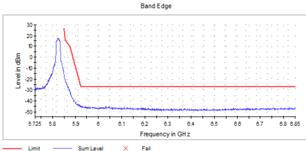
Graph 25: Antenna 1 – Upper Band Edge Channel 165 Transmitting (5825 MHz) - Setting 20
