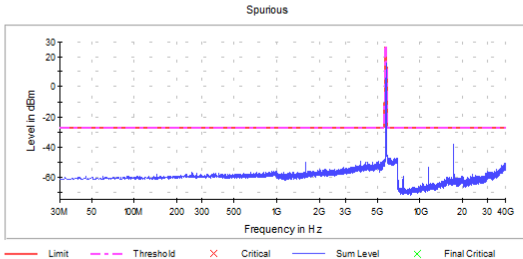
Graph 30: Antenna 1 – Spurious Emissions Channel 157 Transmitting (5785 MHz) - Setting 20
