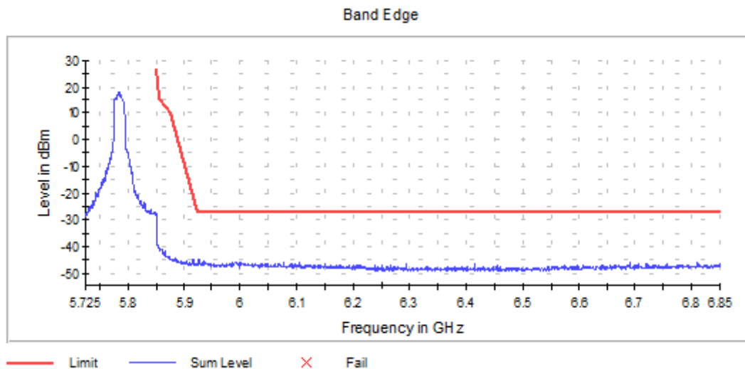
Graph 23: Antenna 1 – Upper Band Edge Channel 157 Transmitting (5785 MHz) - Setting 20
