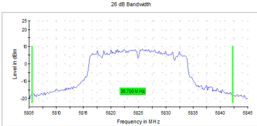
Graph 4: Antenna 0 – 26 dB Emissions Bandwidth Transmitting at 5825 MHz – Setting 20
