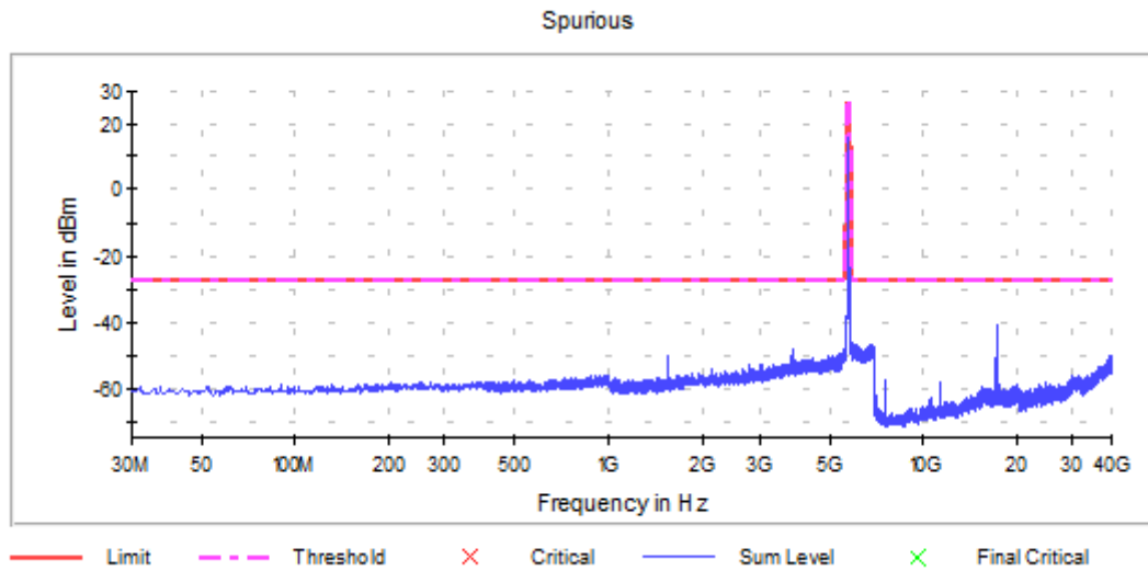
Graph 26: Antenna 0 – Spurious Emissions Channel 149 Transmitting (5745 MHz) - Setting 20
