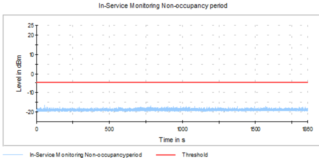
Graph 3: EUTChannel 60 Non-Occupancy Period of 30 minutes.
