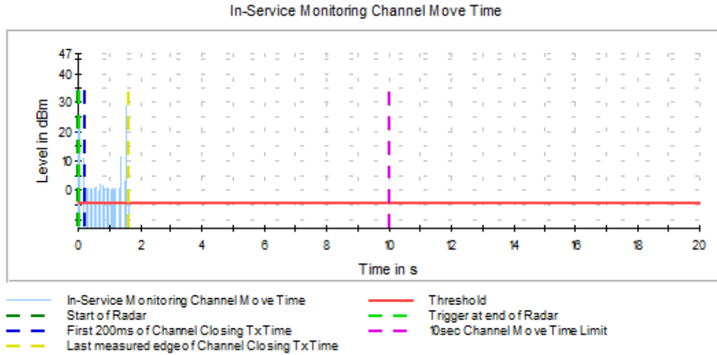
Graph 1: EUT Channel 60 Channel Close Time and Channel Move Time
