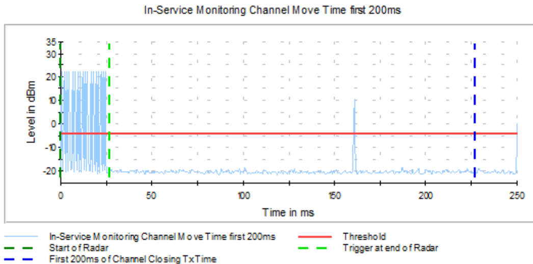
Graph 2: EUT Channel 60 First 200 ms (Channel Closing Tx Time)
