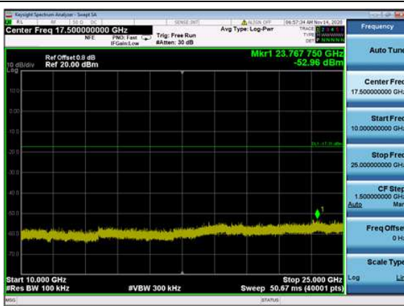
DQPSK,2480MHz,2DH5,Plot 4,10000MHz~25000MHz
