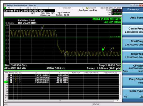
DQPSK,Hopping,2DH5,Band Edge HighRang
