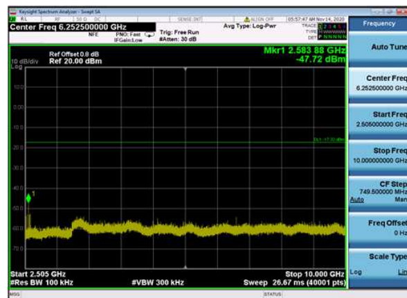
8DPSK,2480MHz,3DH5,Plot 3,2505MHz~10000MHz
