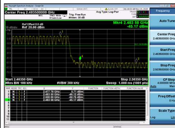
8DPSK,Hopping,3DH5,Band Edge HighRang
