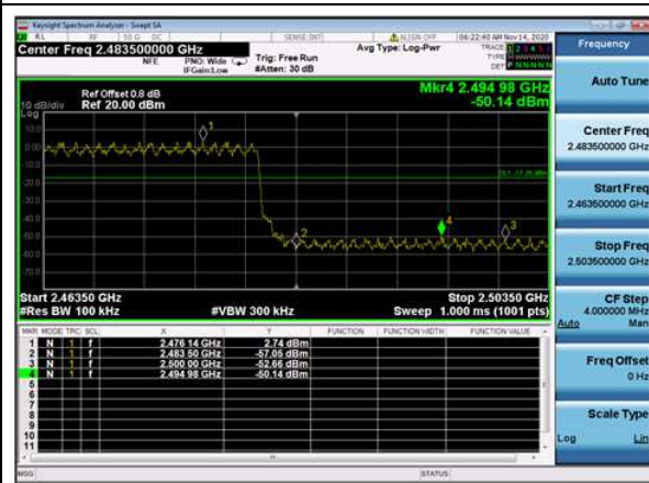
8DPSK,Hopping,3DH5,Band Edge HighRang
