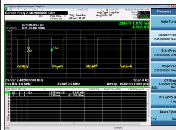
GFSK,2402,DH5,Transmission Time
