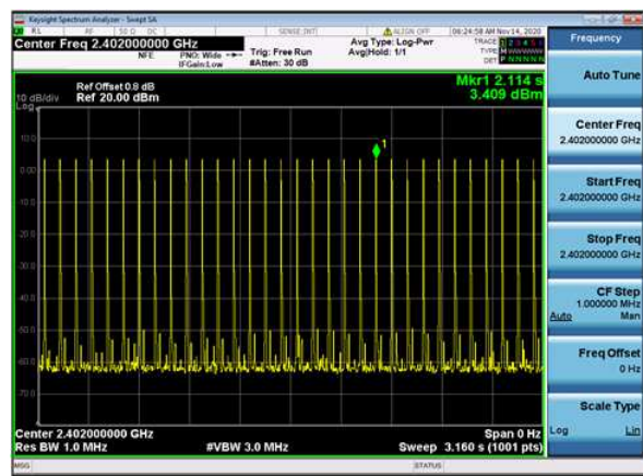
GFSK,2402,DH3,Transmission Number
