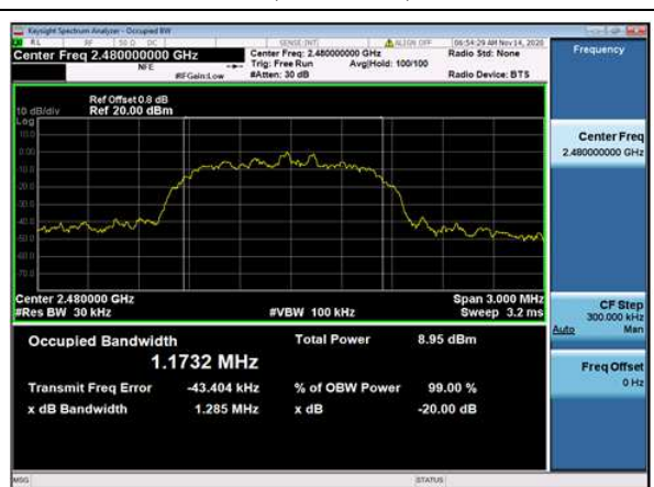
DQPSK,2480MHz,2DH5
