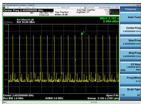
GFSK,2402,DH5,Transmission Number
