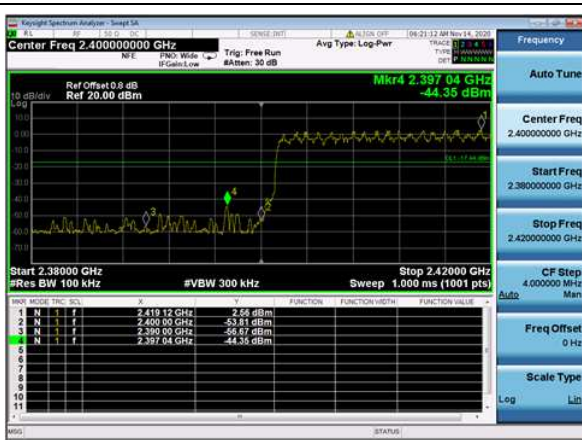
8DPSK,Hopping,3DH5,Band Edge LowRange
