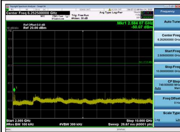
DQPSK,2480MHz,2DH5,Plot 3,2505MHz~10000MHz
