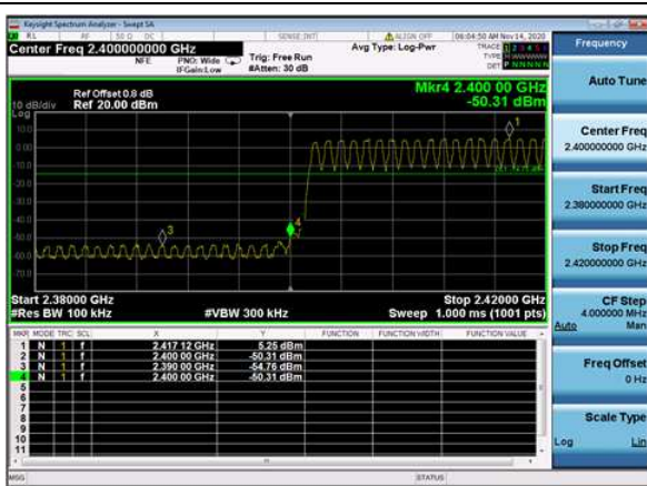
GFSK,Hopping,DH5,Band Edge LowRange
