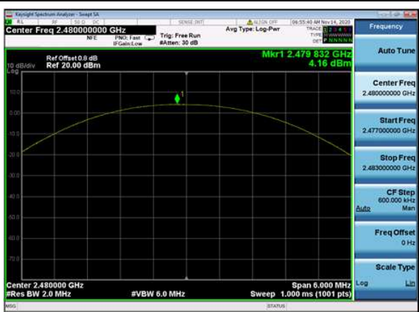
DQPSK,2480MHz,2DH5
