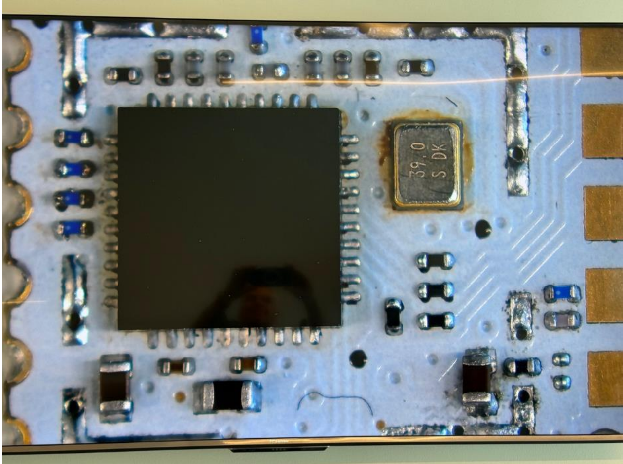
Photograph 1 – View of the RF Circuitry Under the Shield
