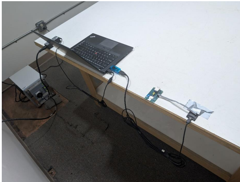
Photograph 7: Back View Conducted Emissions Worst-Case Configuration
