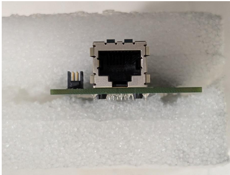
Photograph 11: Bottom View of the EUT in the Host Board
