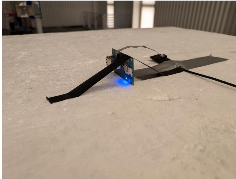
Photograph 3: Closeup of Worst-Case Fundamentals Orientation (Standing Long Edge)
