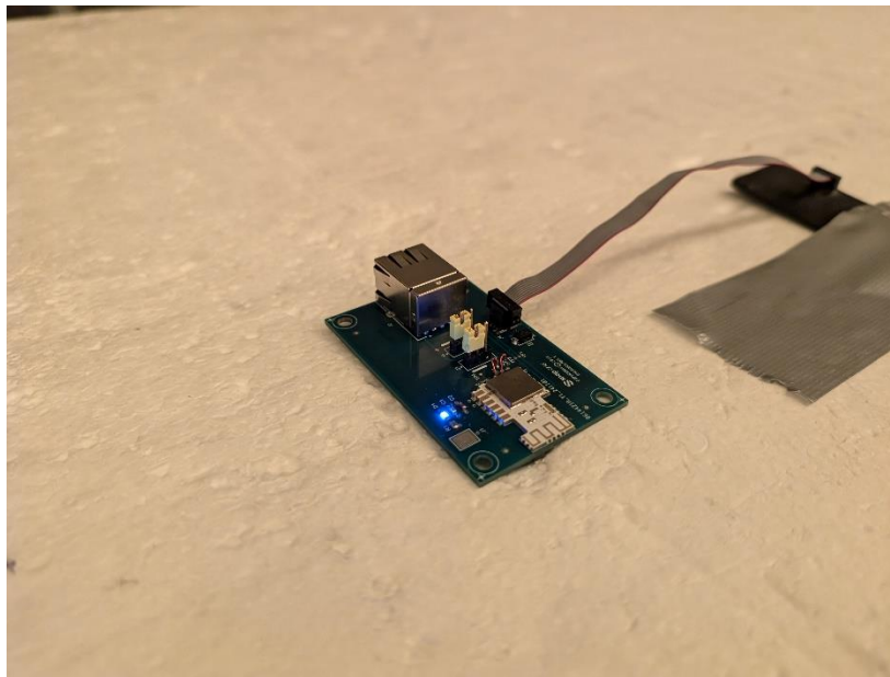
Photograph 4: Closeup of Worst-Case Spurious Orientation (Laying Flat)
