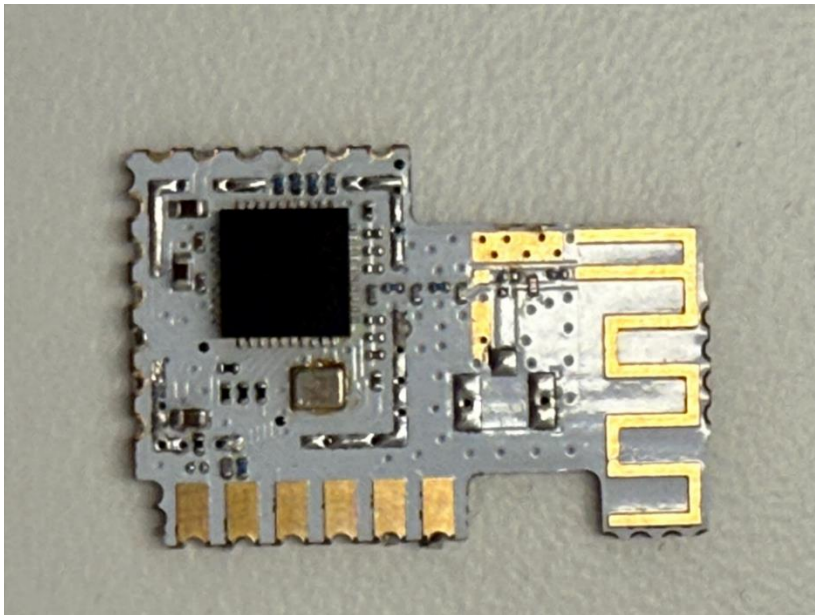
Photograph 20: Front View of the EUT with RF Shell Removed
