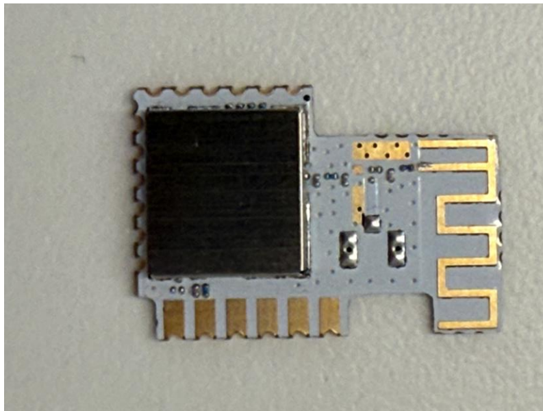
Photograph 14: Front View of the EUT Removed from Host Board
