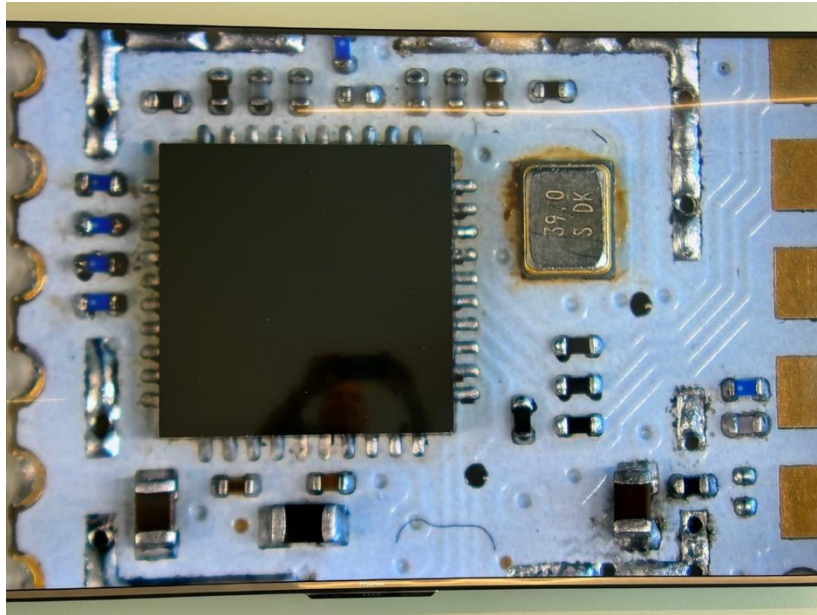
Photograph 21: Closeup View of the EUT with RF Shell Removed
