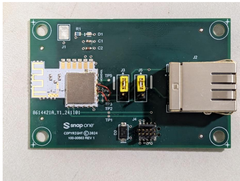
Photograph 8: Front View of the EUT in the Host Board
