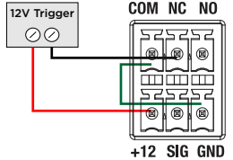
Wire the relay with power from the contact, normally closed (Amplifier trigger)
