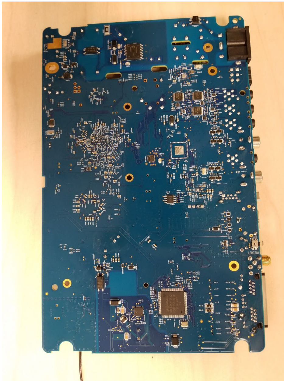
View of the BOTTOM side of the PCB
