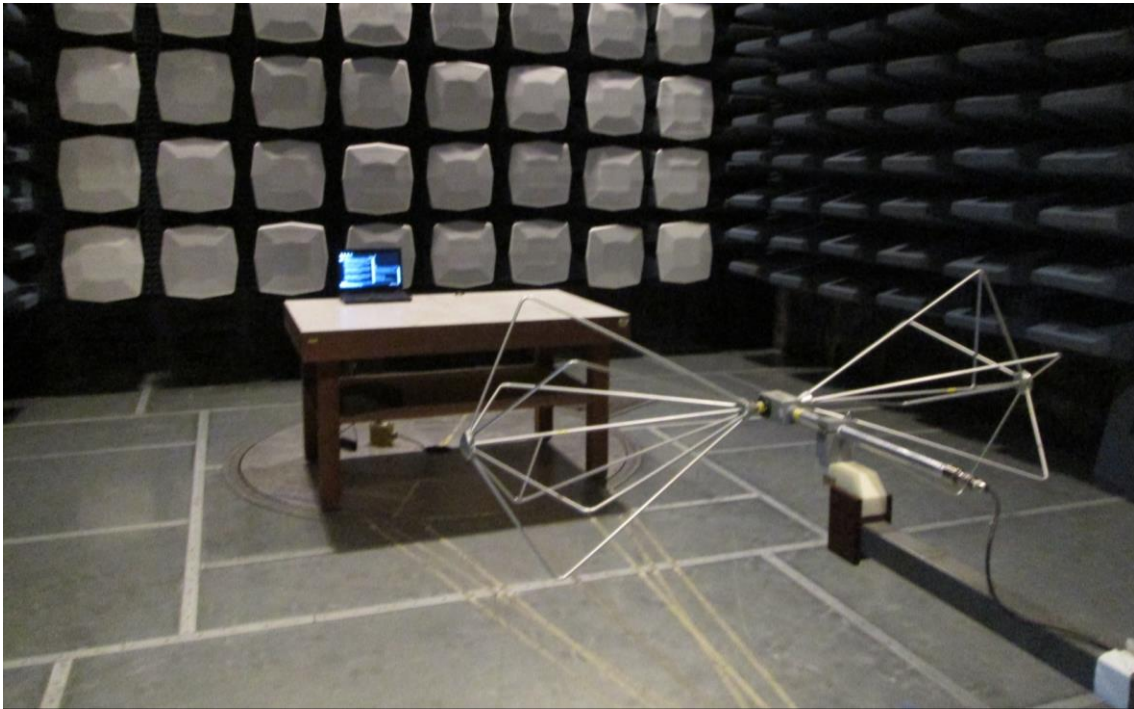
Radiated Emission Test, above 30MHz
