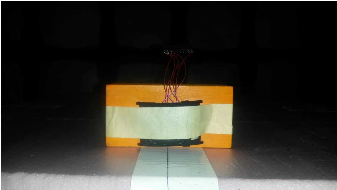
Radiated Emission Test, placement of the EUT
